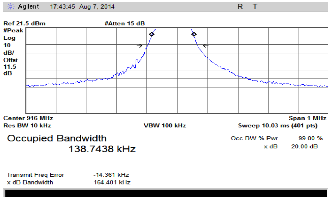
Plot 8 – Middle Channel – 20dB BW (FHSS Mode)
