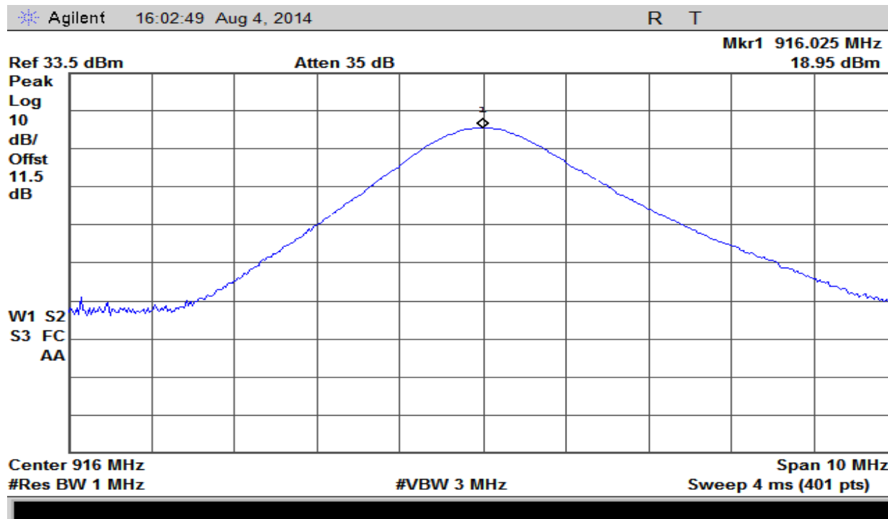
Plot 11 – Output Power – Mid
