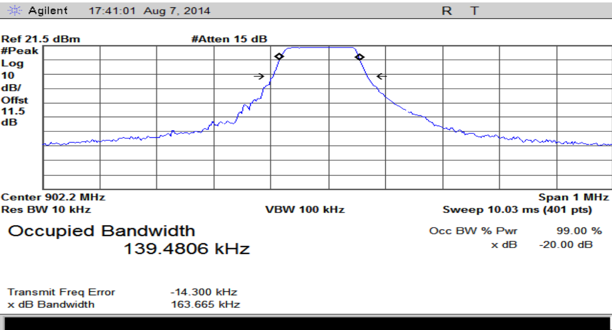
Plot 7 – Lowest Channel – 20dB BW (FHSS Mode)
