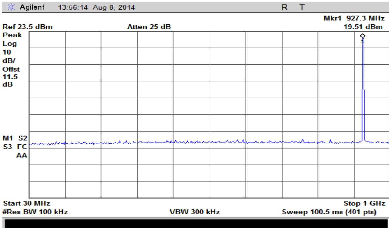
Plot 14 – High Band – 30MHz to 1GHz
