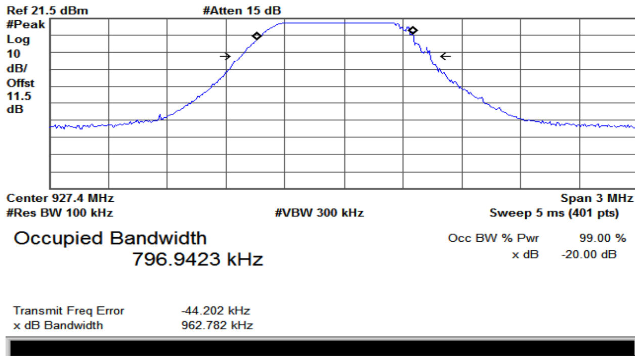
Plot 6 – Highest Channel – 20dB BW
