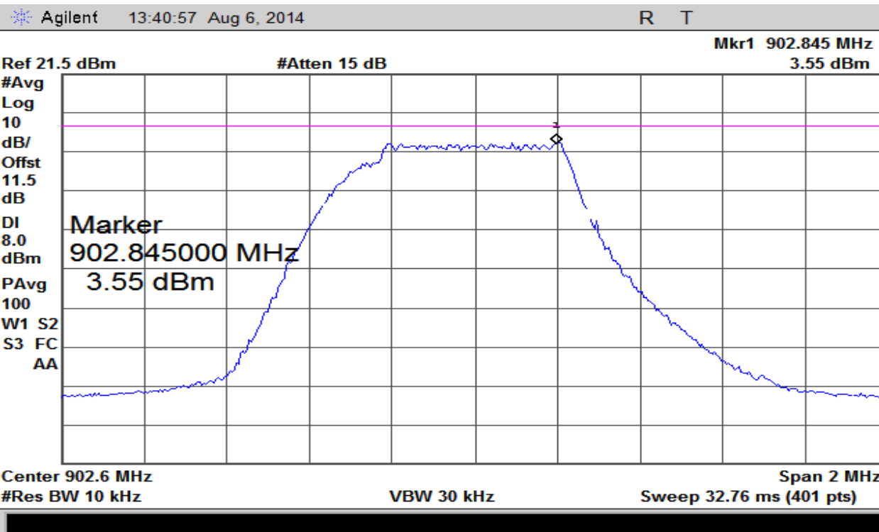
Plot 18 – Power Spectral Density – Lowest Channel
