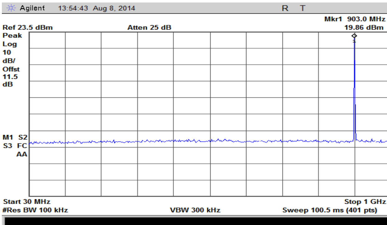
Plot 10 – Low Band – 30MHz to 1GHz
