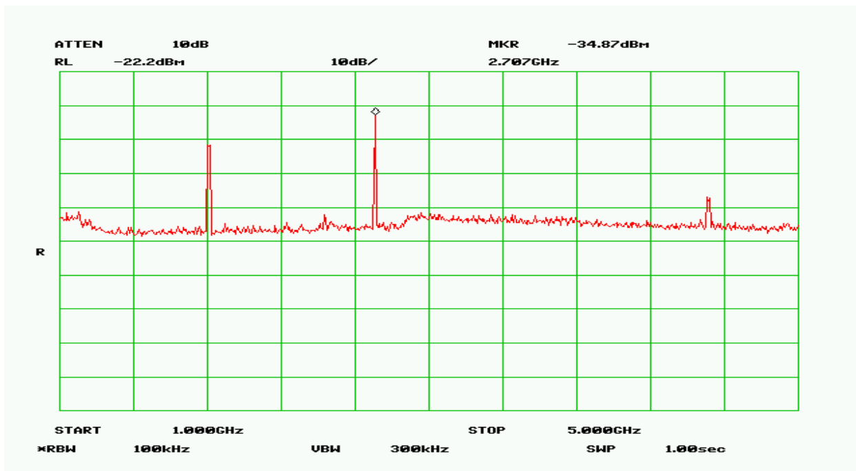
Plot 11 – Low Band – 1GHz to 5GHz
