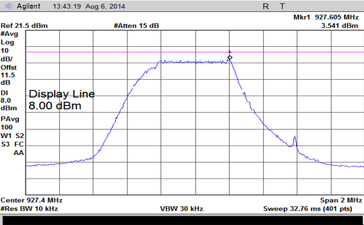
Plot 20 – Power Spectral Density – Highest Channel
