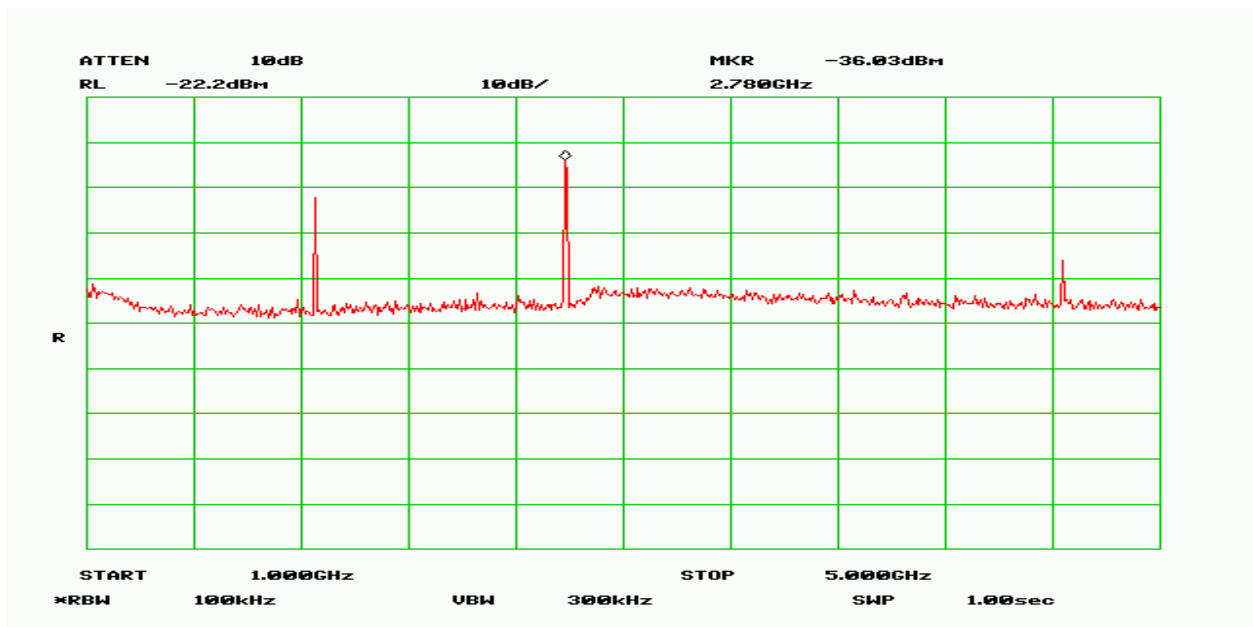
Plot 15 – High Band – 1GHz to 5GHz
