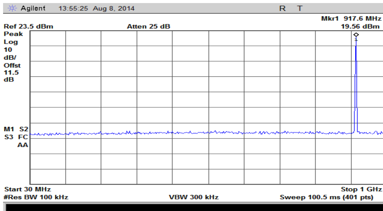
Plot 13 – Mid Band - 30MHz to 1GHz
