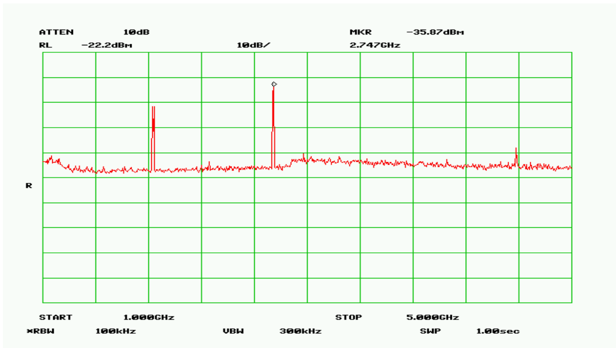
Plot 14 – Mid Band – 1GHz to 5GHz
