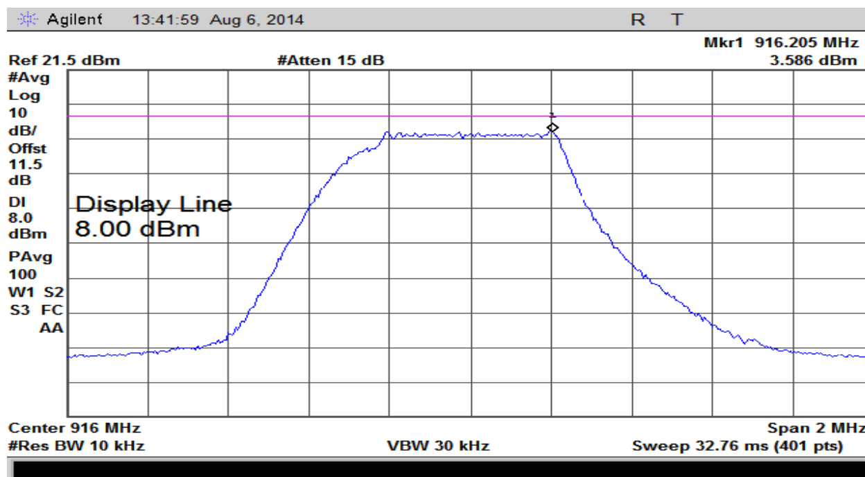
Plot 19 – Power Spectral Density – Middle Channel
