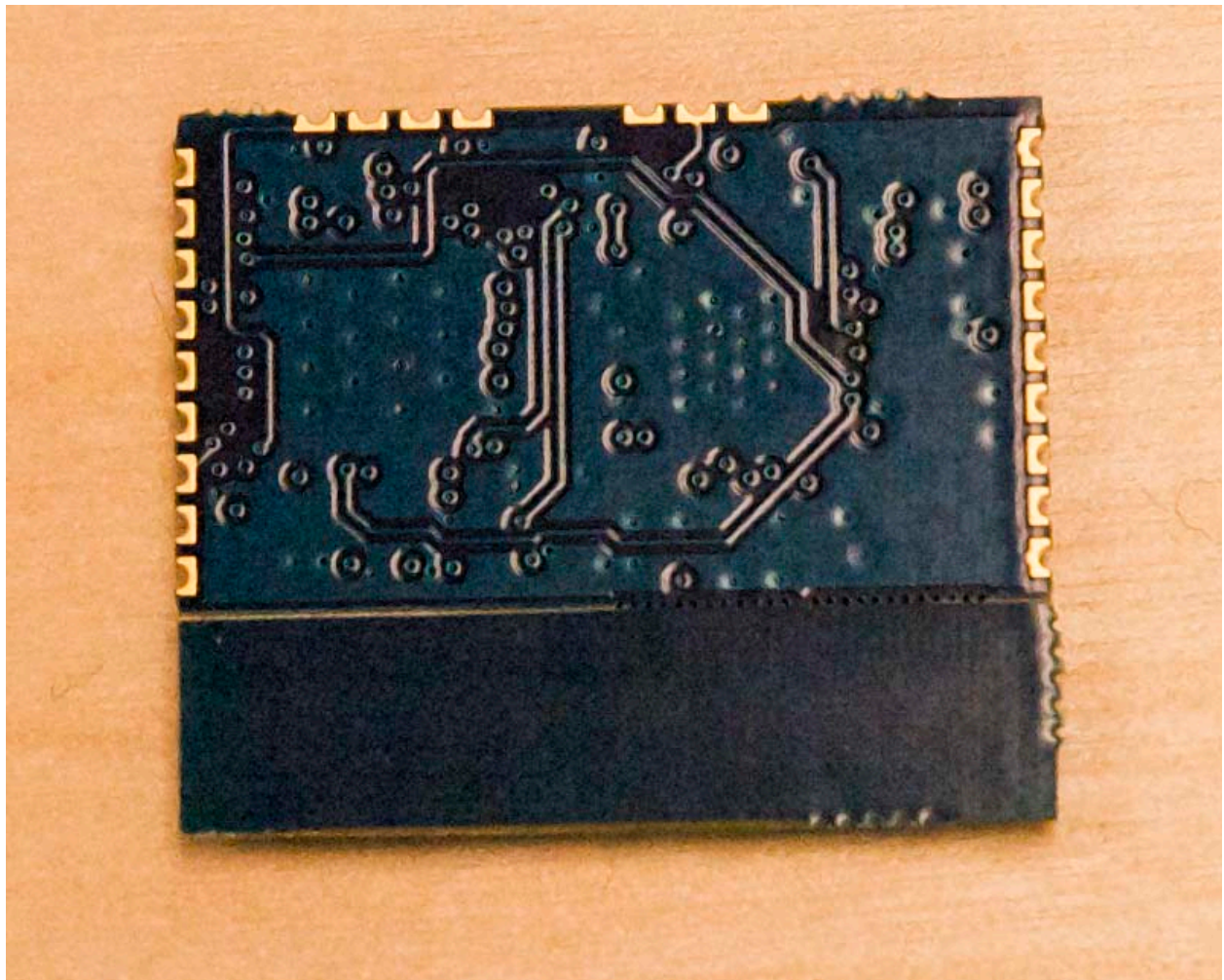
Bottom view of LLRLP20 (with trace antenna)
