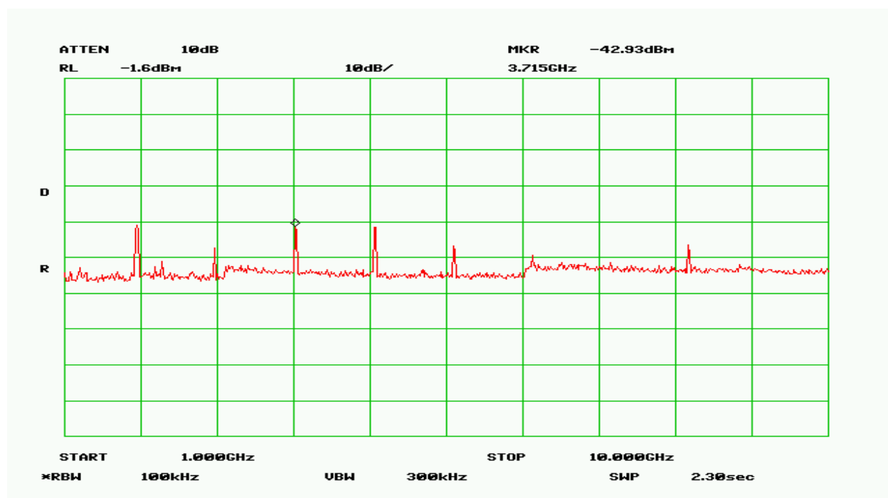
Plot 18 – High Band – 1GHz to 10GHz
