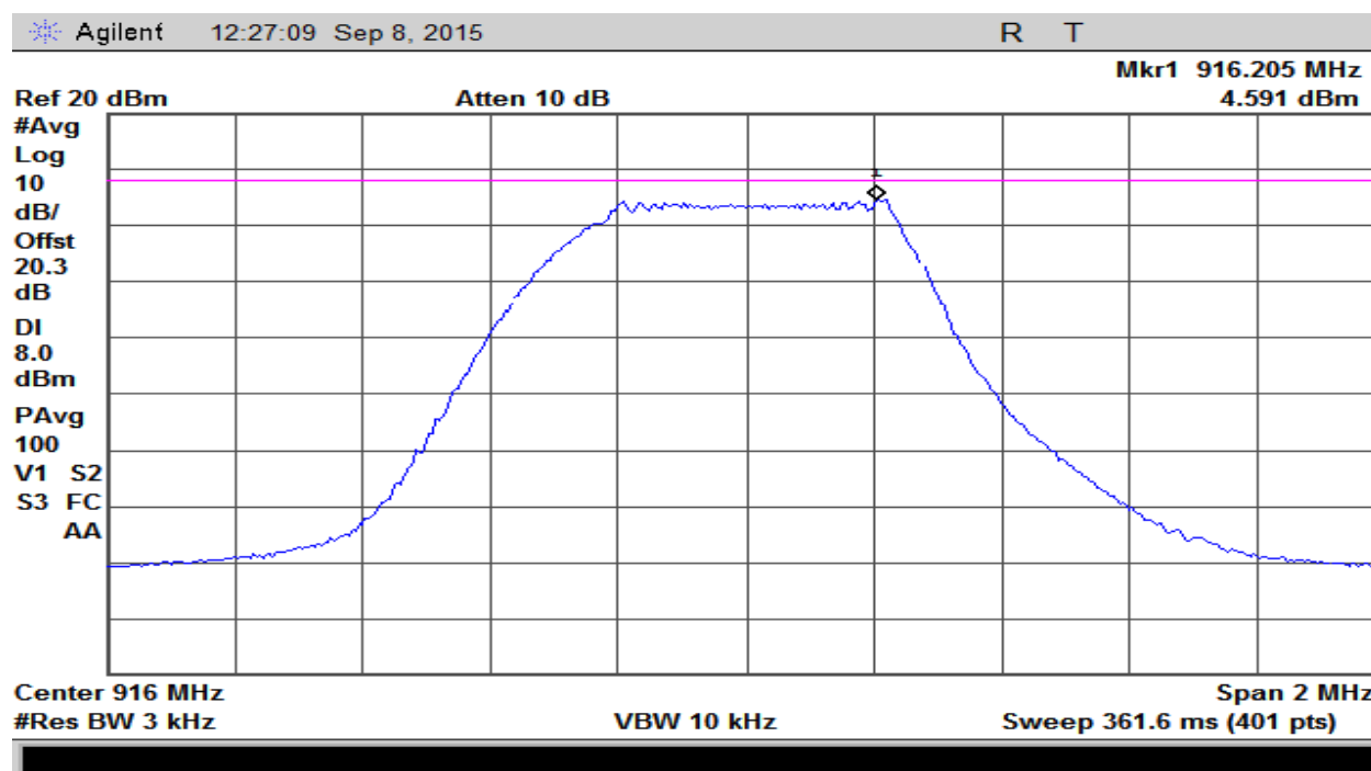
Plot 21 – Power Spectral Density – Middle Channel - DTS Mode
