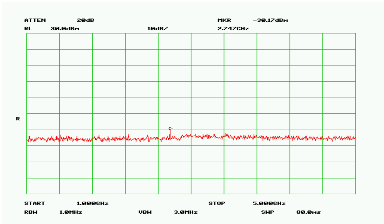
Plot 13 – Mid Band – 1GHz to 5GHz
