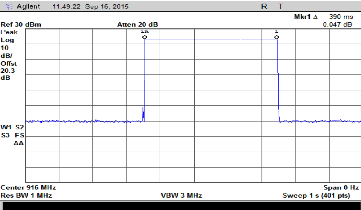
Plot 20 – Dwell Time
