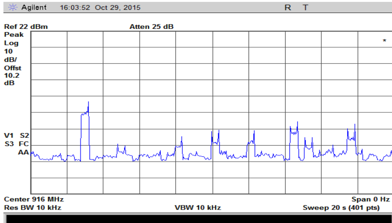
Plot 21 – # of Hops in 20 second period –
