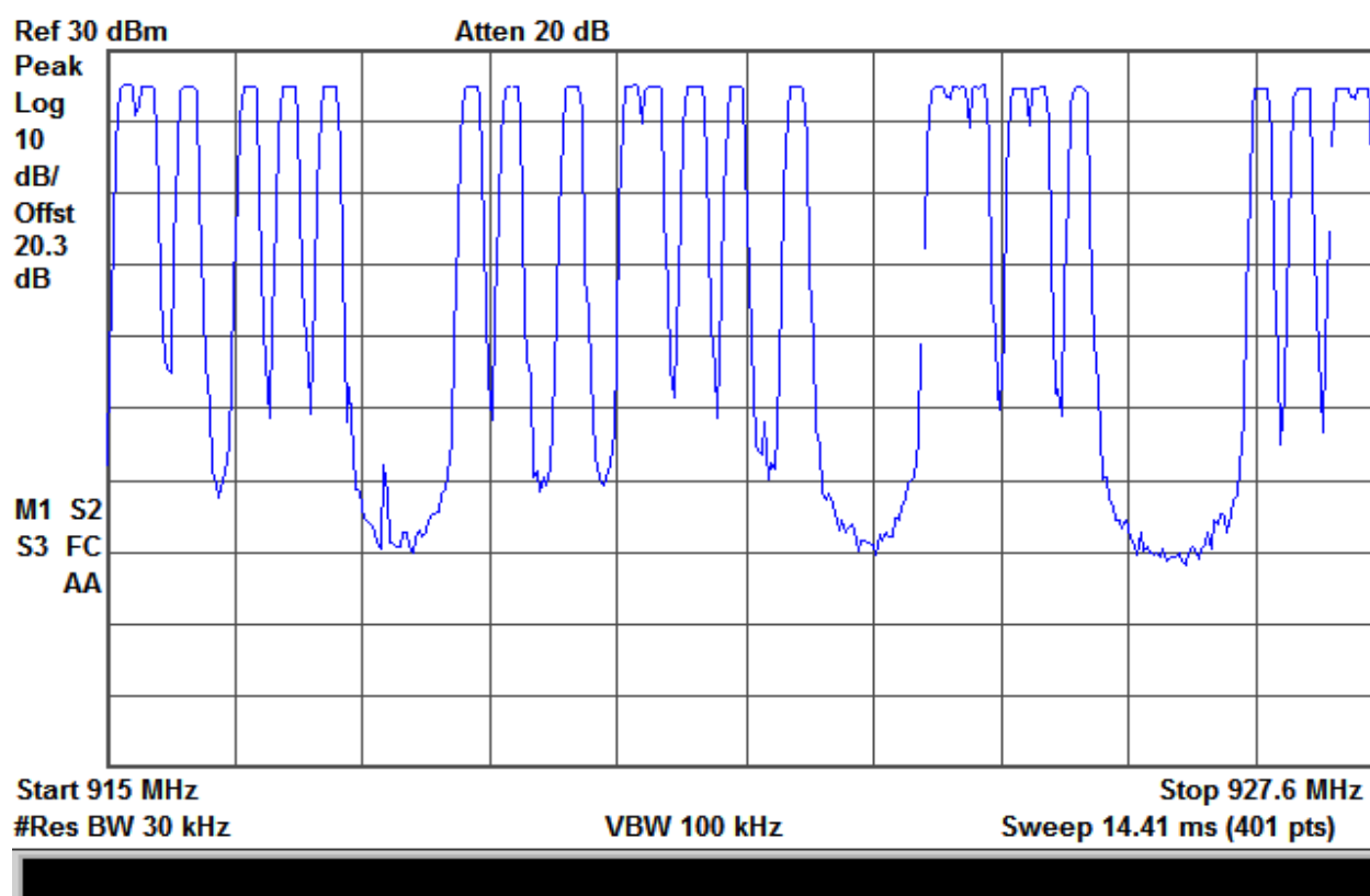
Plot 23 – Number of Frequency Hops – 915MHz to 927.6MHz
