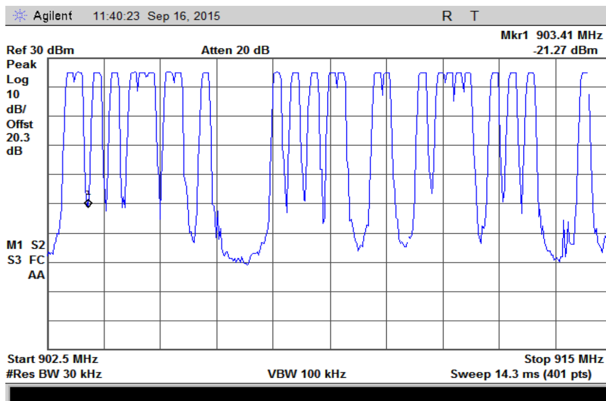
Plot 22 – Number of Frequency Hops – 902.5MHz to 915MHz
