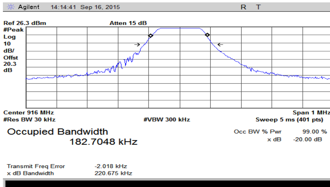
Plot 4 – Middle Channel – 20dB BW (FHSS Mode)
