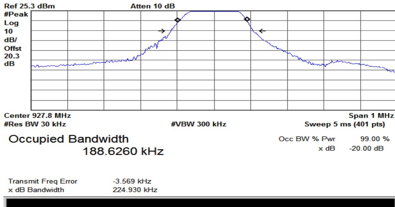
Plot 5 – Highest Channel – 20dB BW (FHSS Mode)
