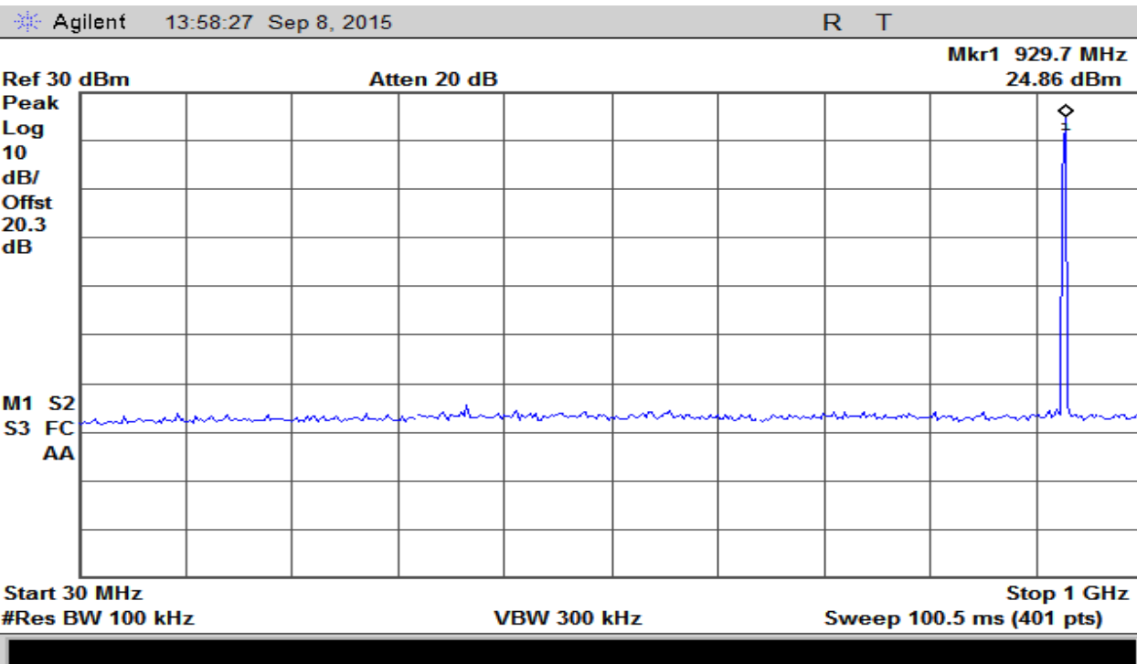
Plot 15 – High Band – 30MHz to 1GHz
