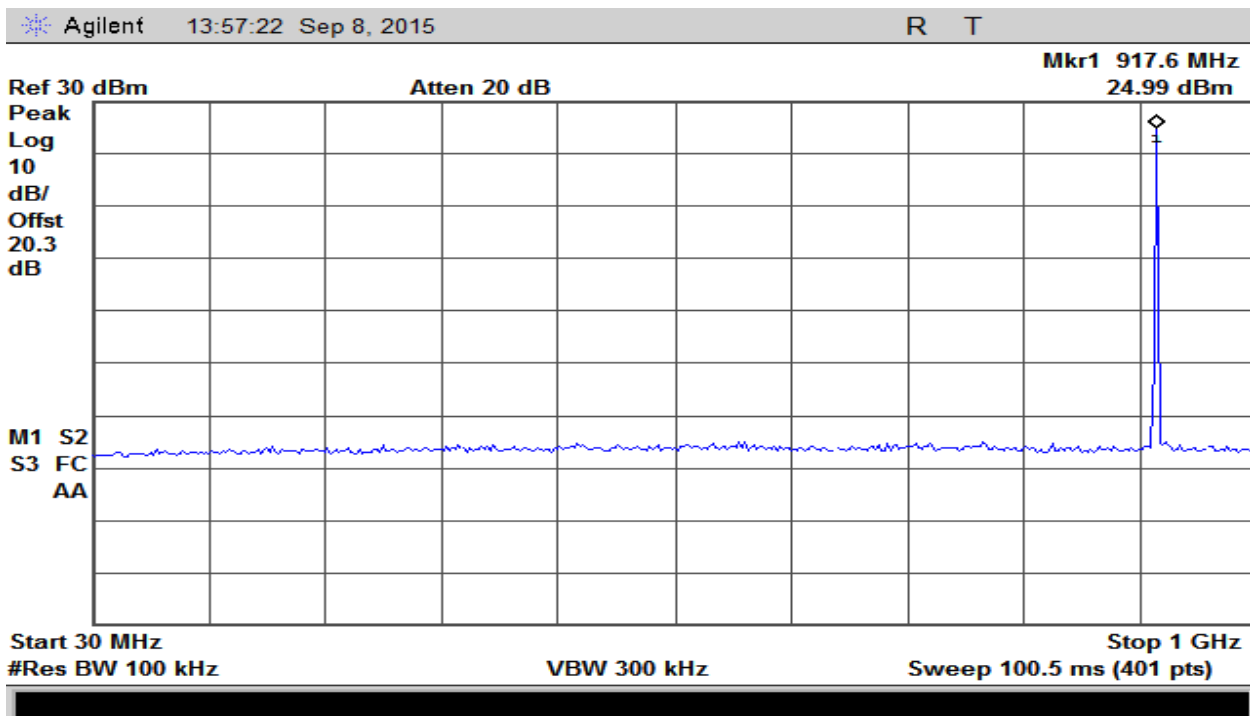
Plot 12 – Mid Band – 30MHz to 1GHz
