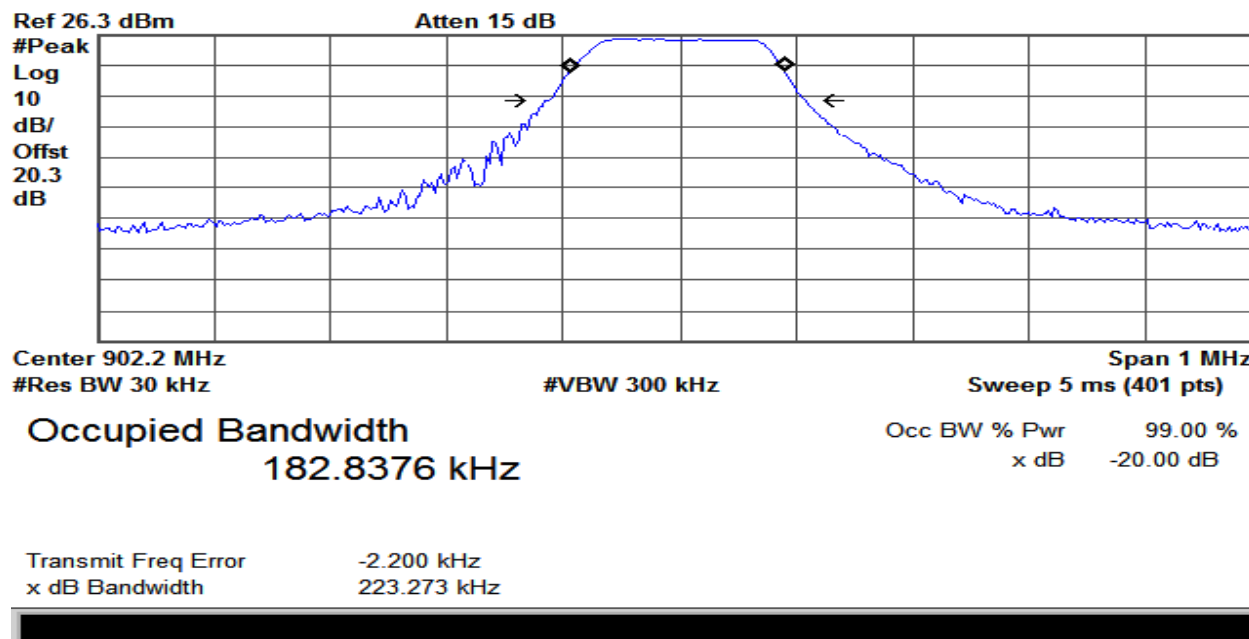
Plot 3 – Lowest Channel – 20dB BW (FHSS Mode)
