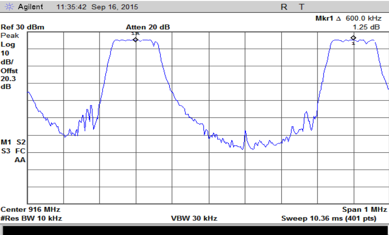
Plot 24 – Carrier Frequency Separation (Using Delta Marker Method)
