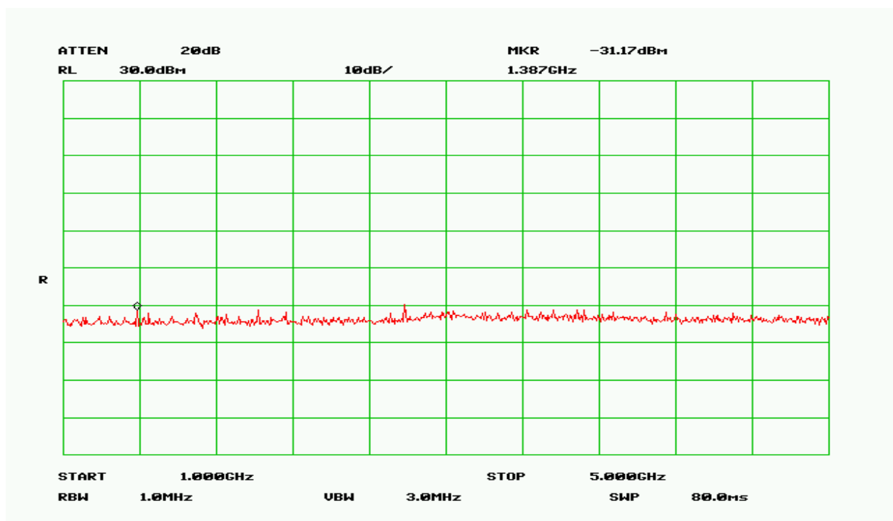
Plot 16 – High Band – 1GHz to 5GHz
