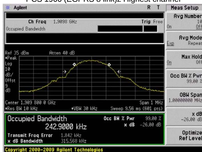
PCS 1900 (EGPRS 8 link)z Highest channel
