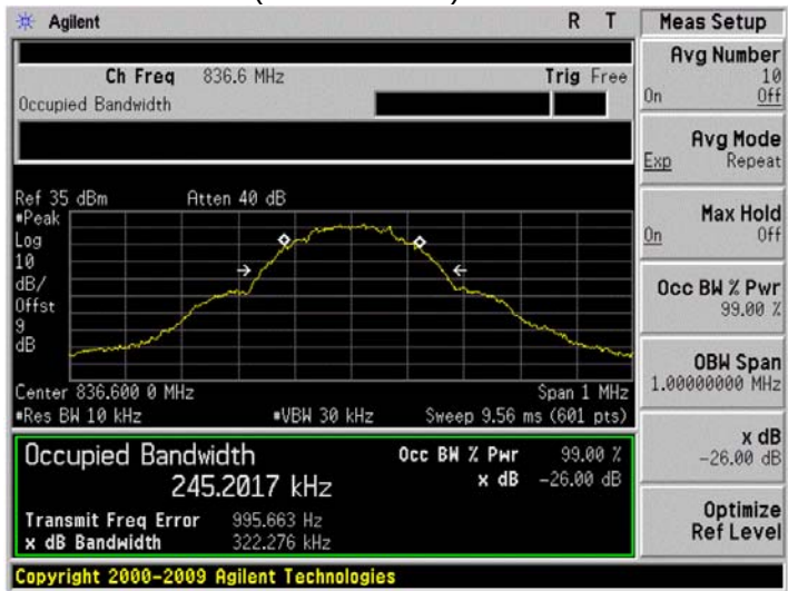
GSM 850 (EGPRS 8 link) Middle channel
