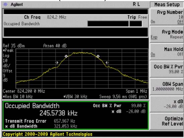
GSM 850 (EGPRS 8 link) Lowest channel
