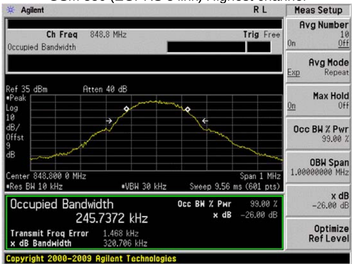
GSM 850 (EGPRS 8 link) Highest channel
