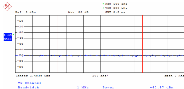
Highest channel
