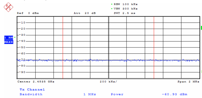
Highest channel
