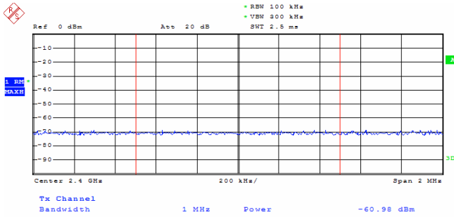
Lowest channel
