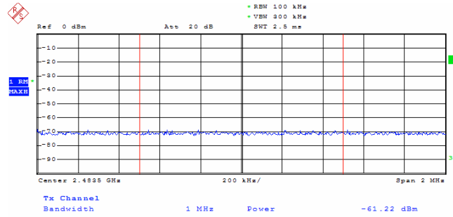
Highest channel
