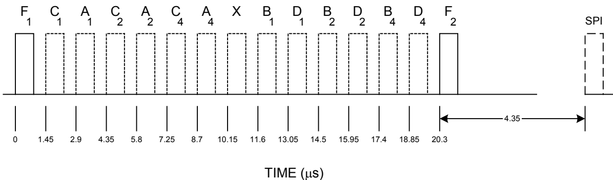
Figure 3: ATCRBS Reply
