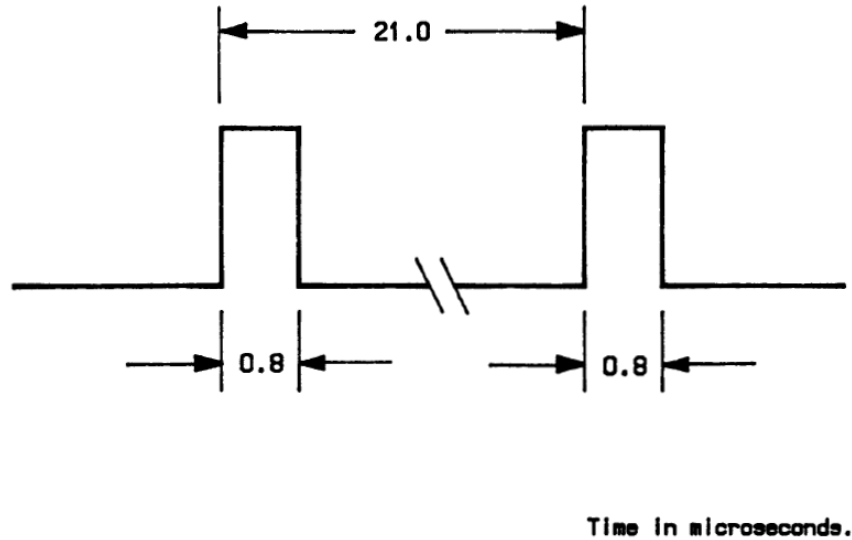
Figure 2 ATCRBS Mode C Interrogation
