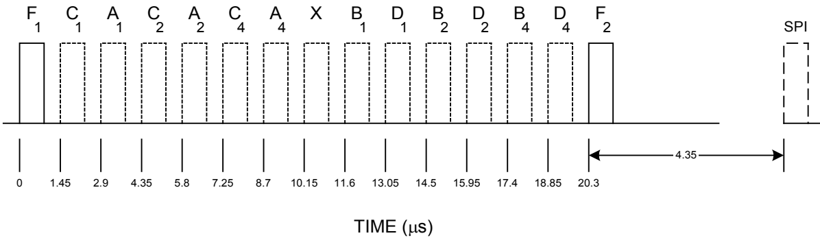
Figure 1: ATCRBS Reply
