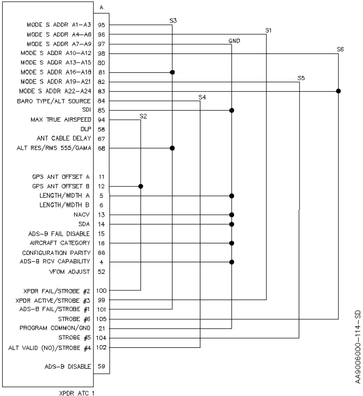
Figure 4-1: Example of Configuration Encoding Pinout (N6754H)
