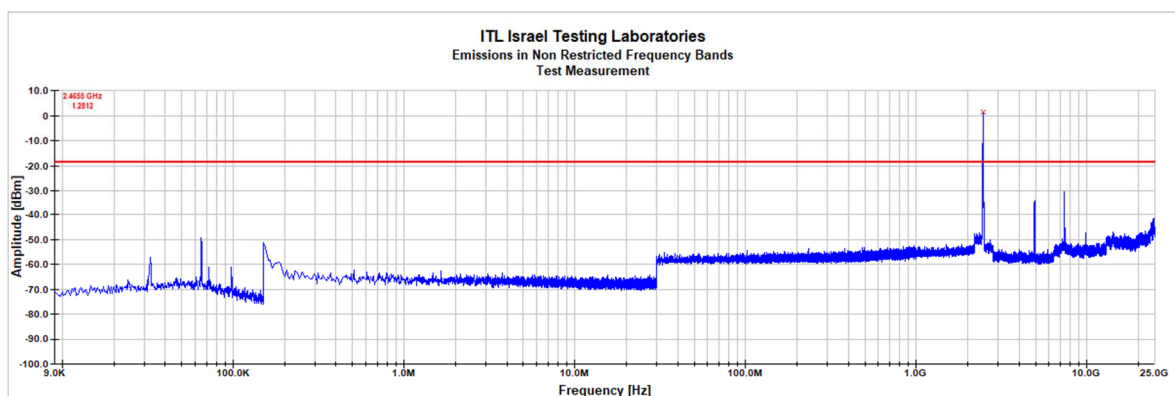
Figure 122 2462.0 MHz, WI-FI/g(6Mbit/s)
