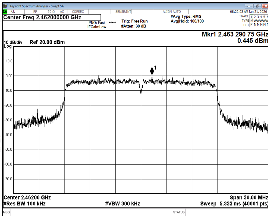
Tx. Spurious NVNT n20 2462MHz Ant1 Ref
