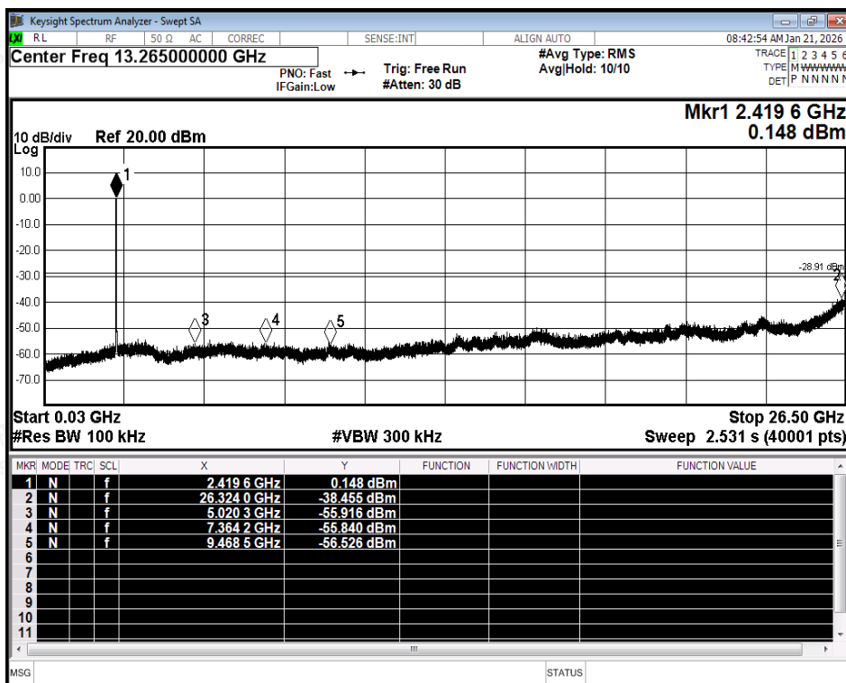
Tx. Spurious NVNT ax20 2412MHz Ant1 Emission
