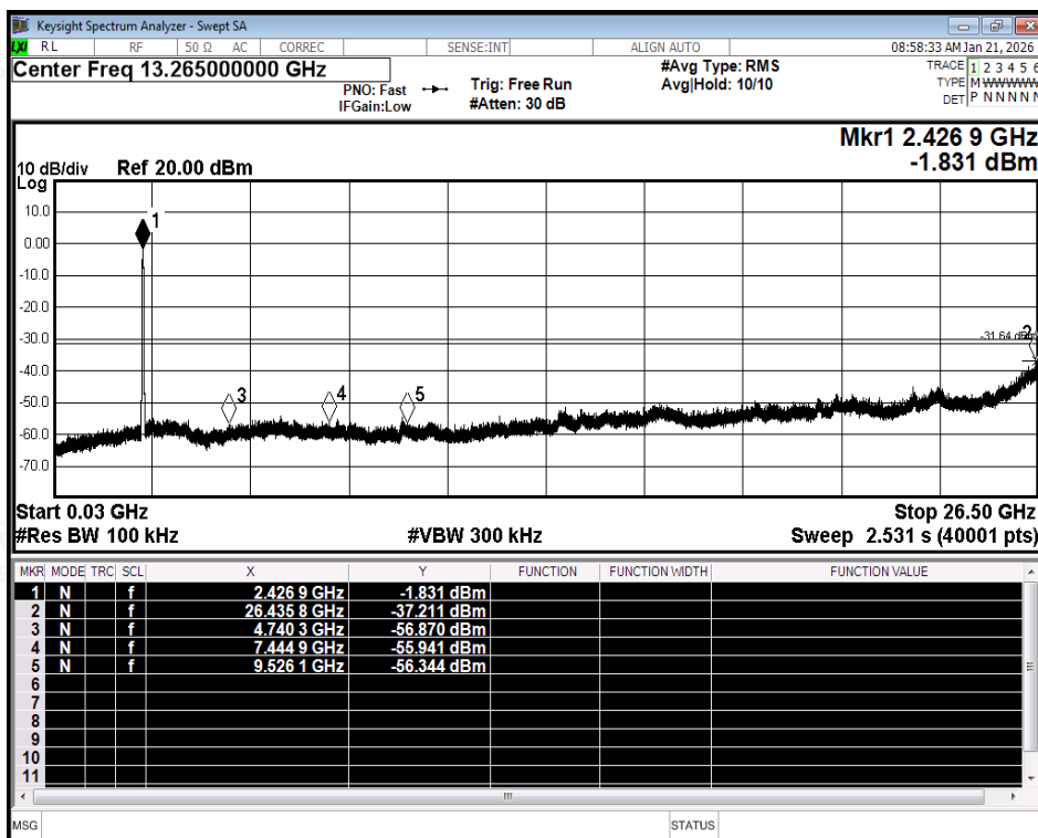
Tx. Spurious NVNT ax40 2422MHz Ant1 Emission
