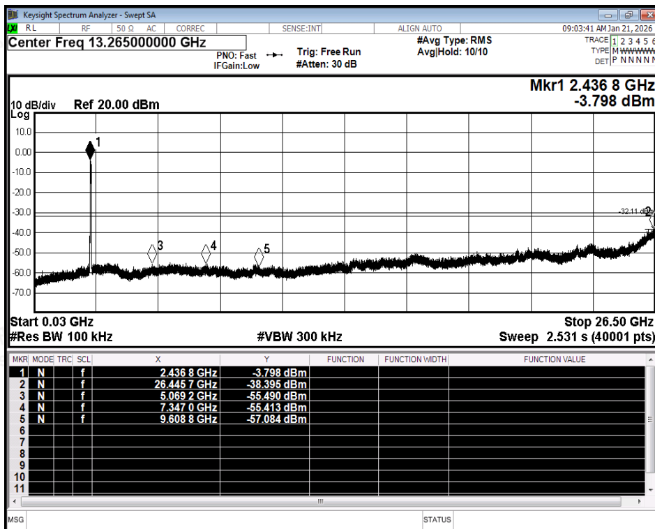
Tx. Spurious NVNT ax40 2452MHz Ant1 Emission
