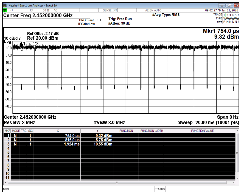
Duty Cycle NVNT ax40 2452MHz Ant1
