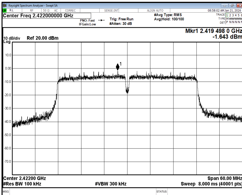
Tx. Spurious NVNT ax40 2422MHz Ant1 Ref
