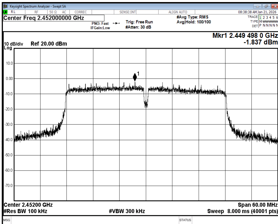
Tx. Spurious NVNT n40 2452MHz Ant1 Ref
