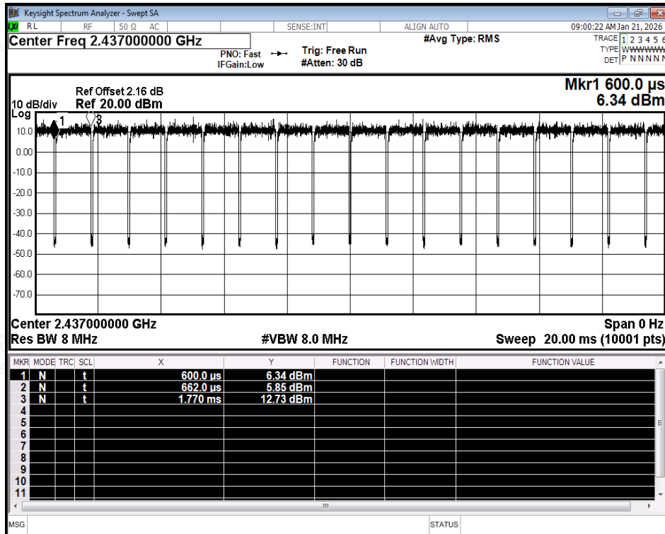
Duty Cycle NVNT ax40 2437MHz Ant1
