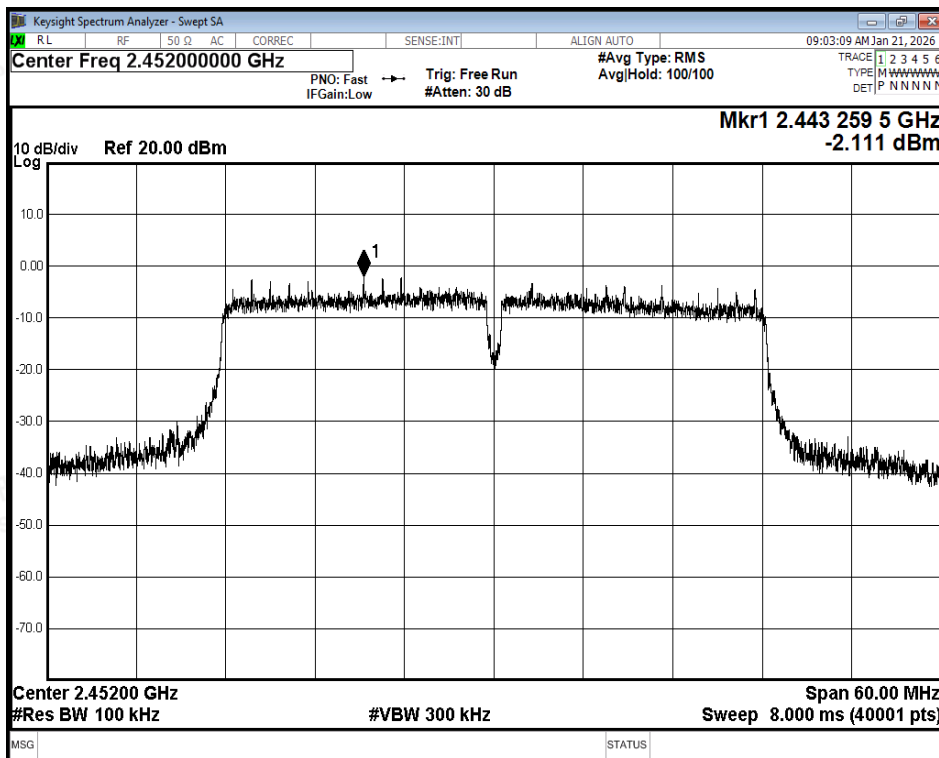
Tx. Spurious NVNT ax40 2452MHz Ant1 Ref
