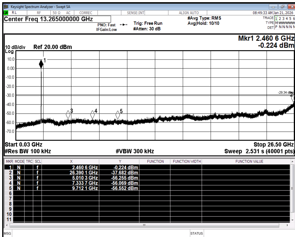
Tx. Spurious NVNT ax20 2462MHz Ant1 Emission
