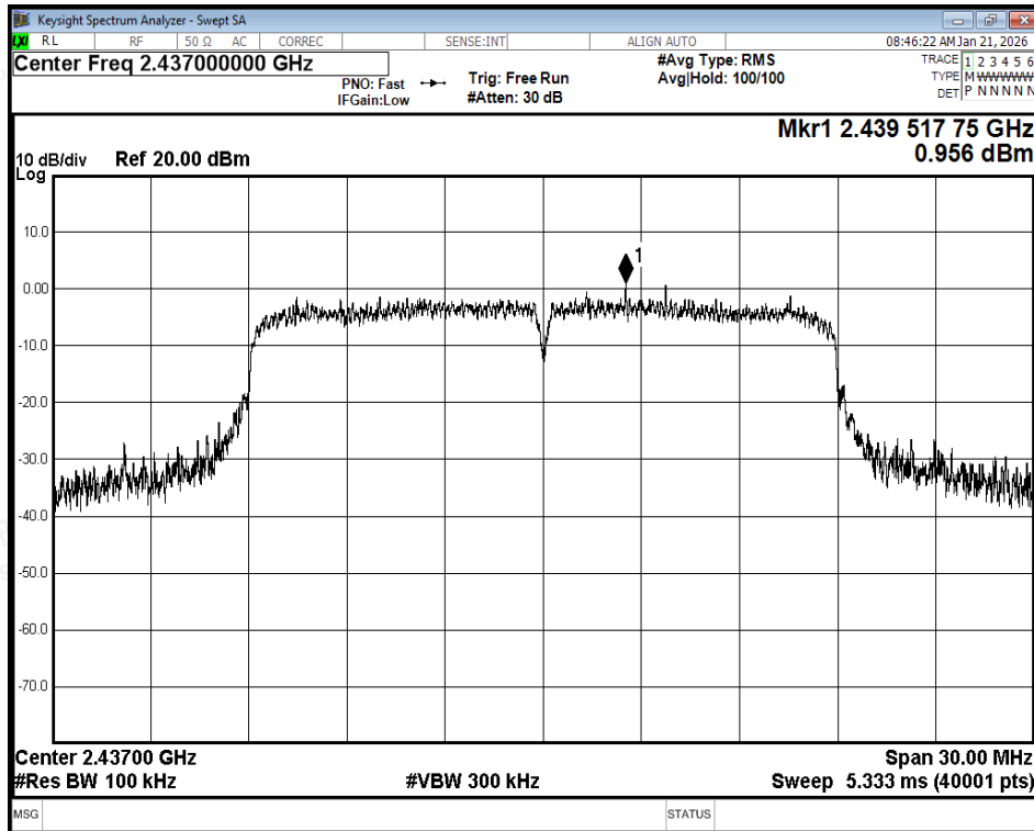
Tx. Spurious NVNT ax20 2437MHz Ant1 Ref
