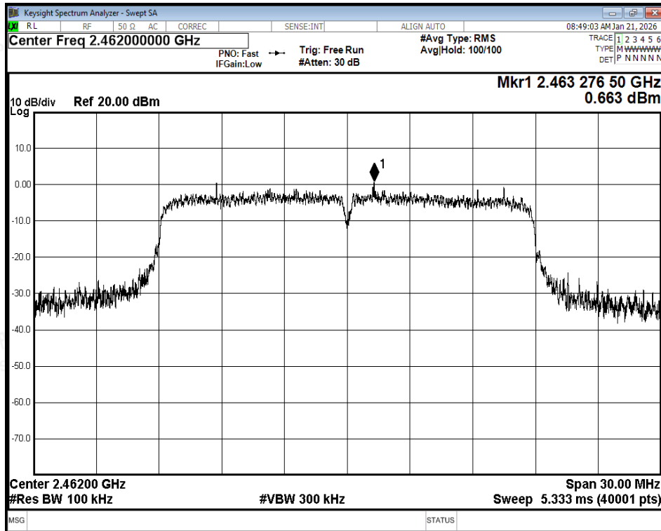
Tx. Spurious NVNT ax20 2462MHz Ant1 Ref
