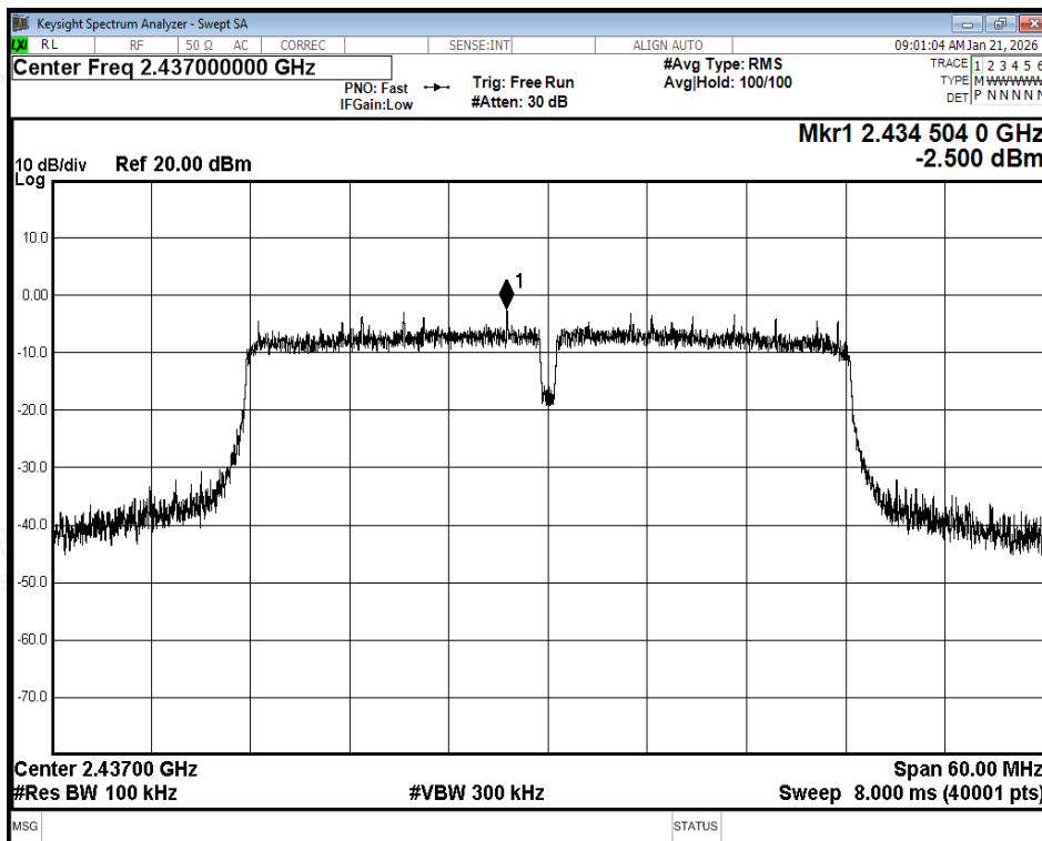
Tx. Spurious NVNT ax40 2437MHz Ant1 Ref
