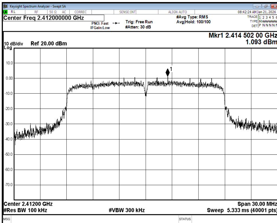
Tx. Spurious NVNT ax20 2412MHz Ant1 Ref
