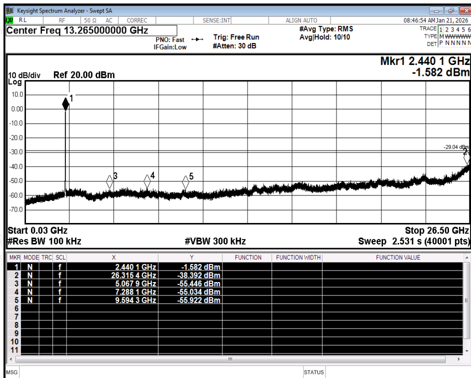
Tx. Spurious NVNT ax20 2437MHz Ant1 Emission
