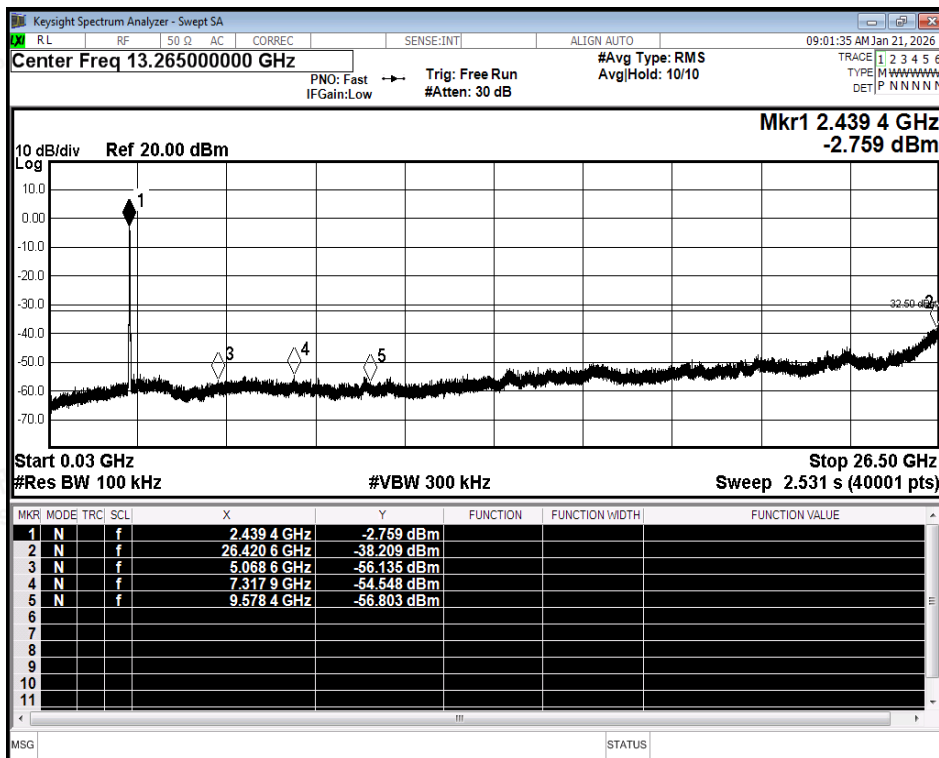
Tx. Spurious NVNT ax40 2437MHz Ant1 Emission
