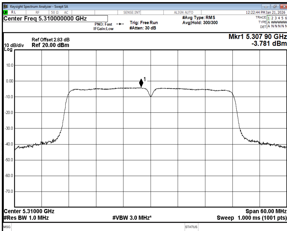
PSD NVNT n40 5310MHz Ant2
