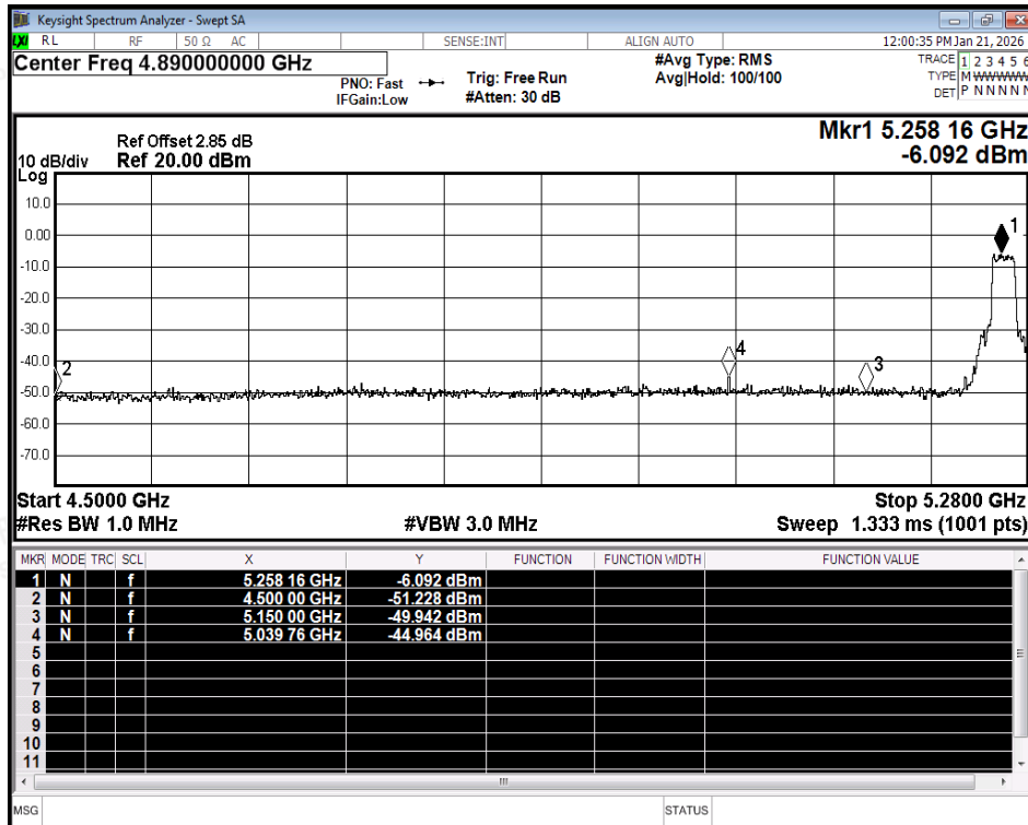
Restrict Band NVNT ac20 5260MHz Ant2 Peak
