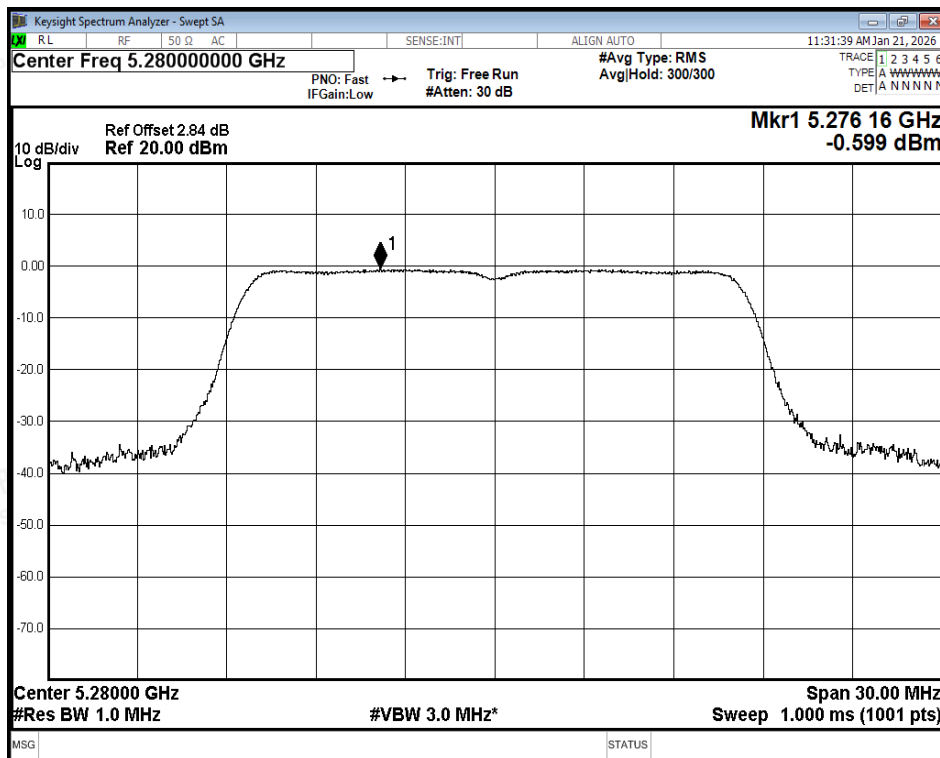
PSD NVNT a 5280MHz Ant2
