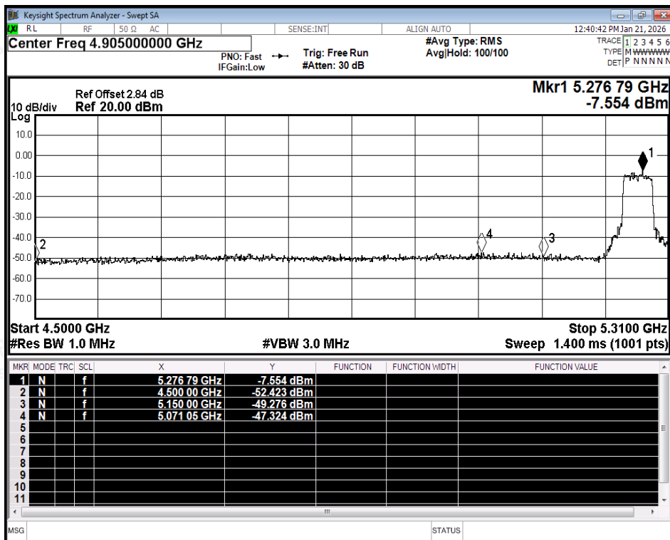
Restrict Band NVNT ac40 5270MHz Ant2 Peak
