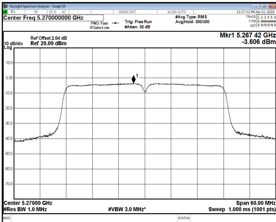
PSD NVNT n40 5270MHz Ant2
