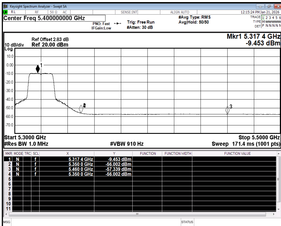
Restrict Band NVNT ax20 5320MHz Ant2 Average
