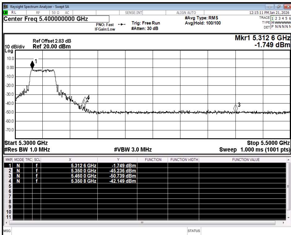
Restrict Band NVNT ax20 5320MHz Ant2 Peak
