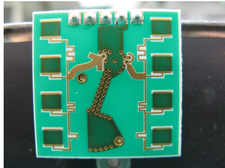
Back side: Patch Antenna
