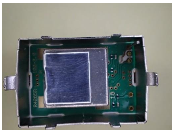
RF circuit: Front side
