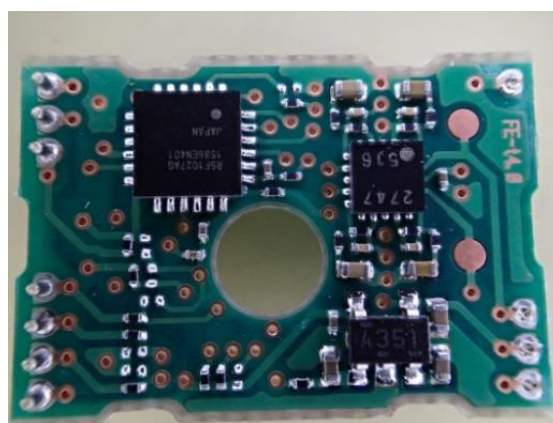
IF circuit: Back side
