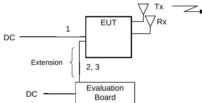
Figure 1: Block Diagram for Radiated Emission of Transmitter
