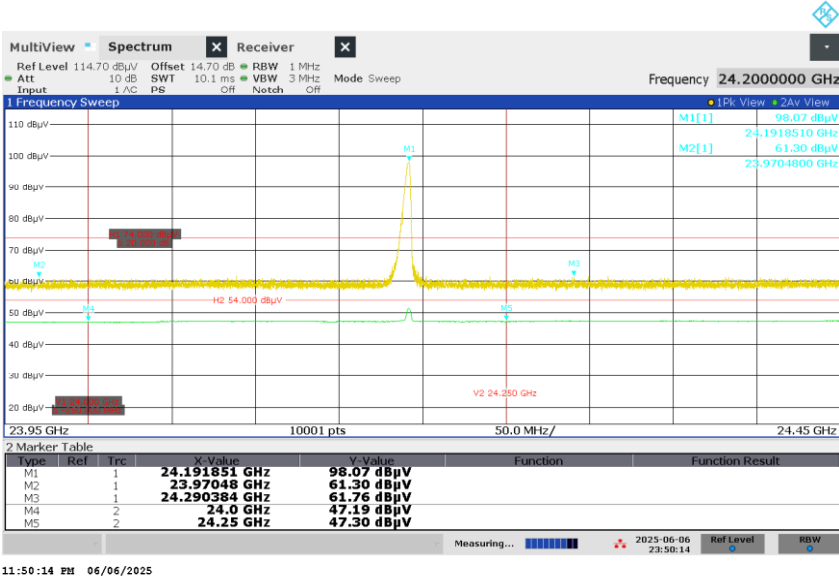
Figure 10: Radiated Emissions at Band Edge, Spectral Diagram, Mode A at Configuration 2
