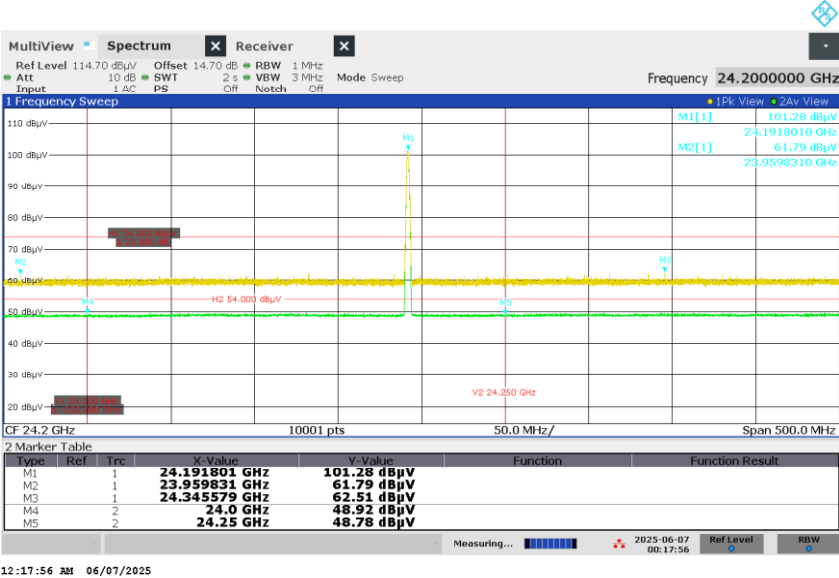
Figure 9: Radiated Emissions at Band Edge, Spectral Diagram, Mode A at Configuration 1
