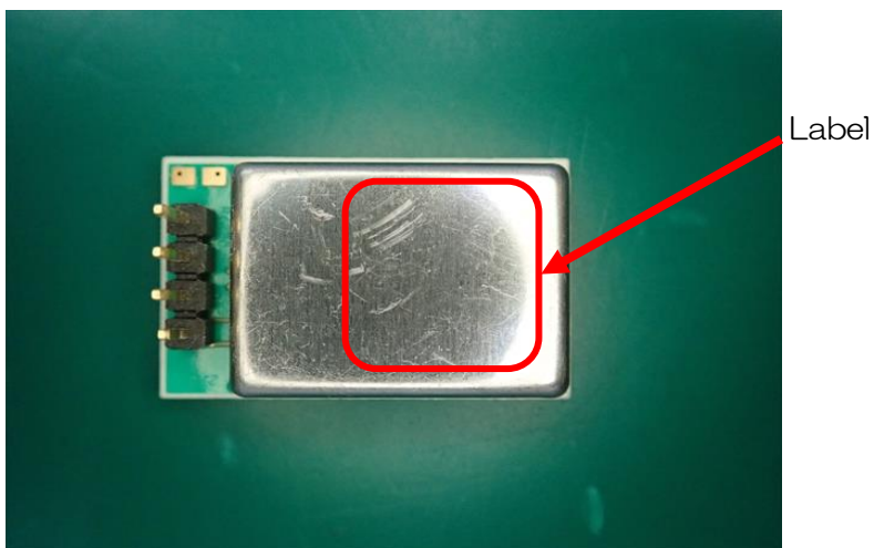
Back Side view: Metal Shielding Cover
