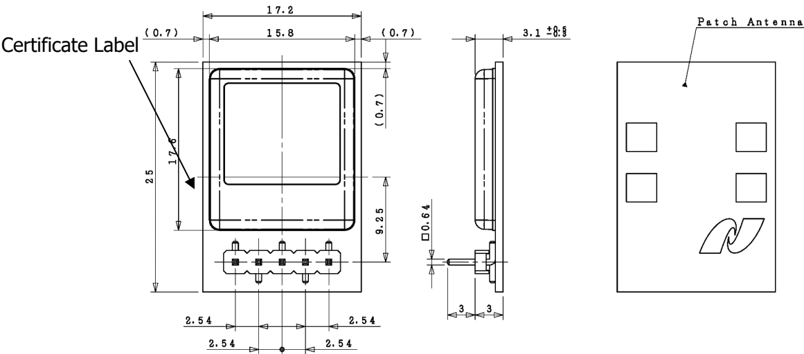
Fig. 4 NJR4267F3B1 Outline drawing
