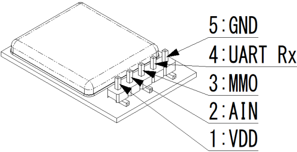
Fig. 5 Pinout Diagram
