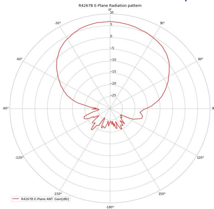
Radiation Pattern
