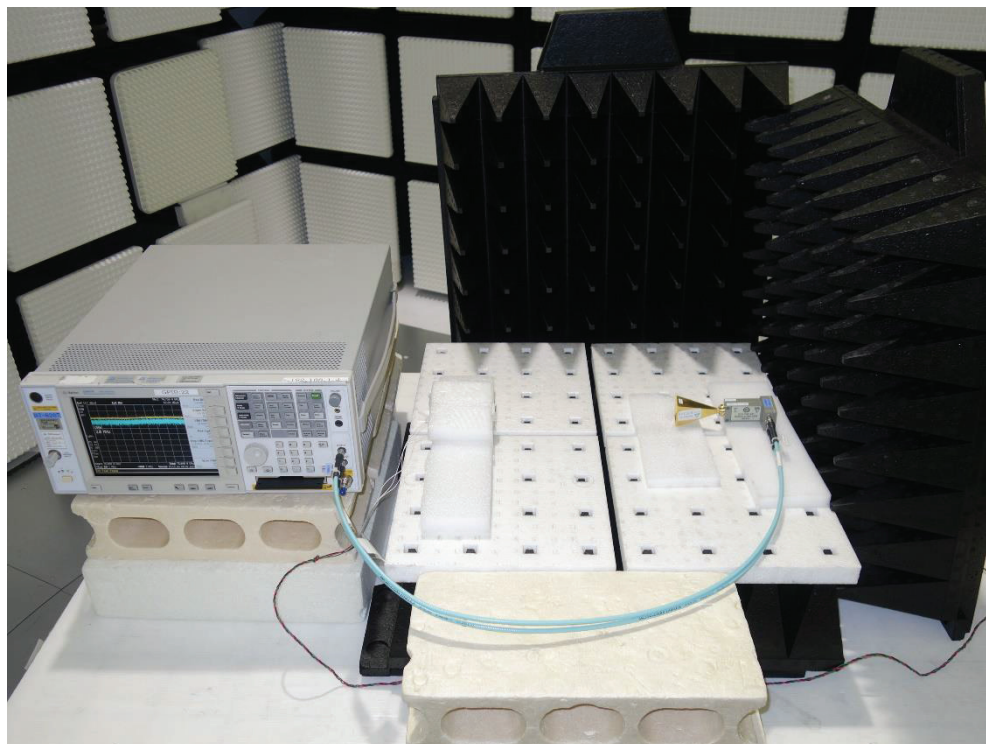
Photograph 7: Set-up for Radiated Emission above 40GHz, Front View
