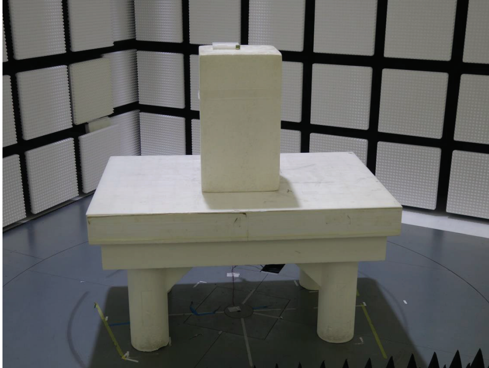
Photograph 5: Set-up for Radiated Emission above 1GHz, Front View
