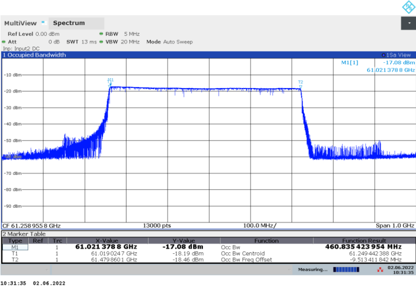
Figure 9: 99% Bandwidth, Mode D3
