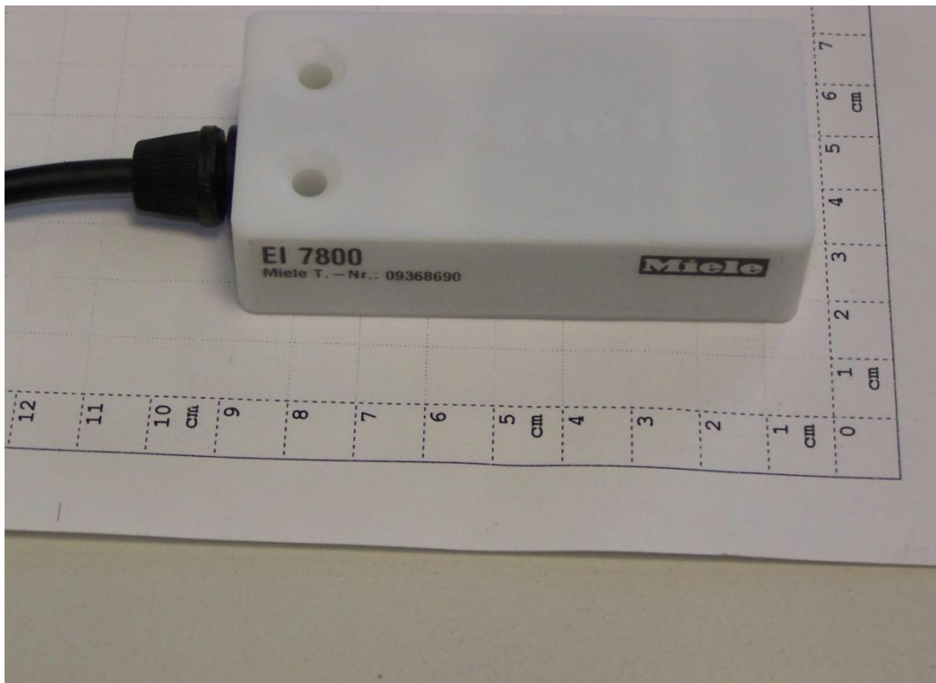
EUT housing case, top and side view
