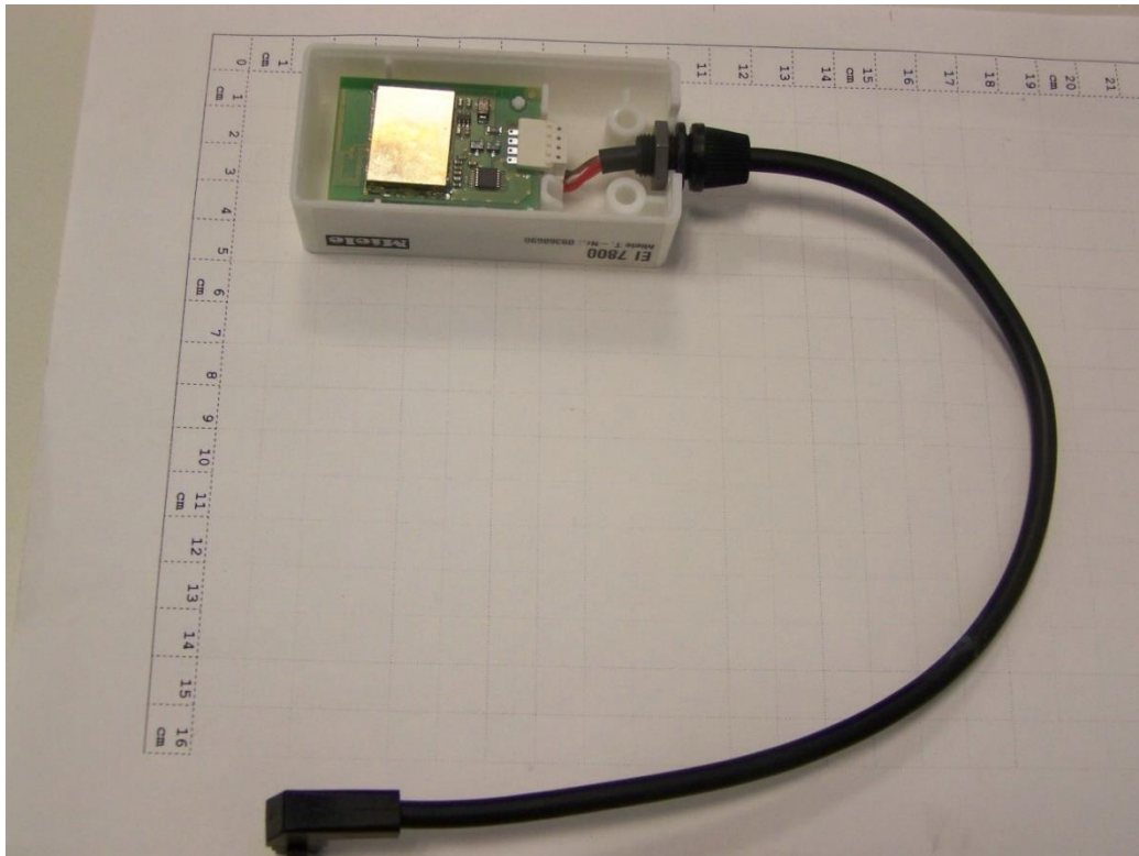
EUT C + Cable 1 connected with open case , top and side view
