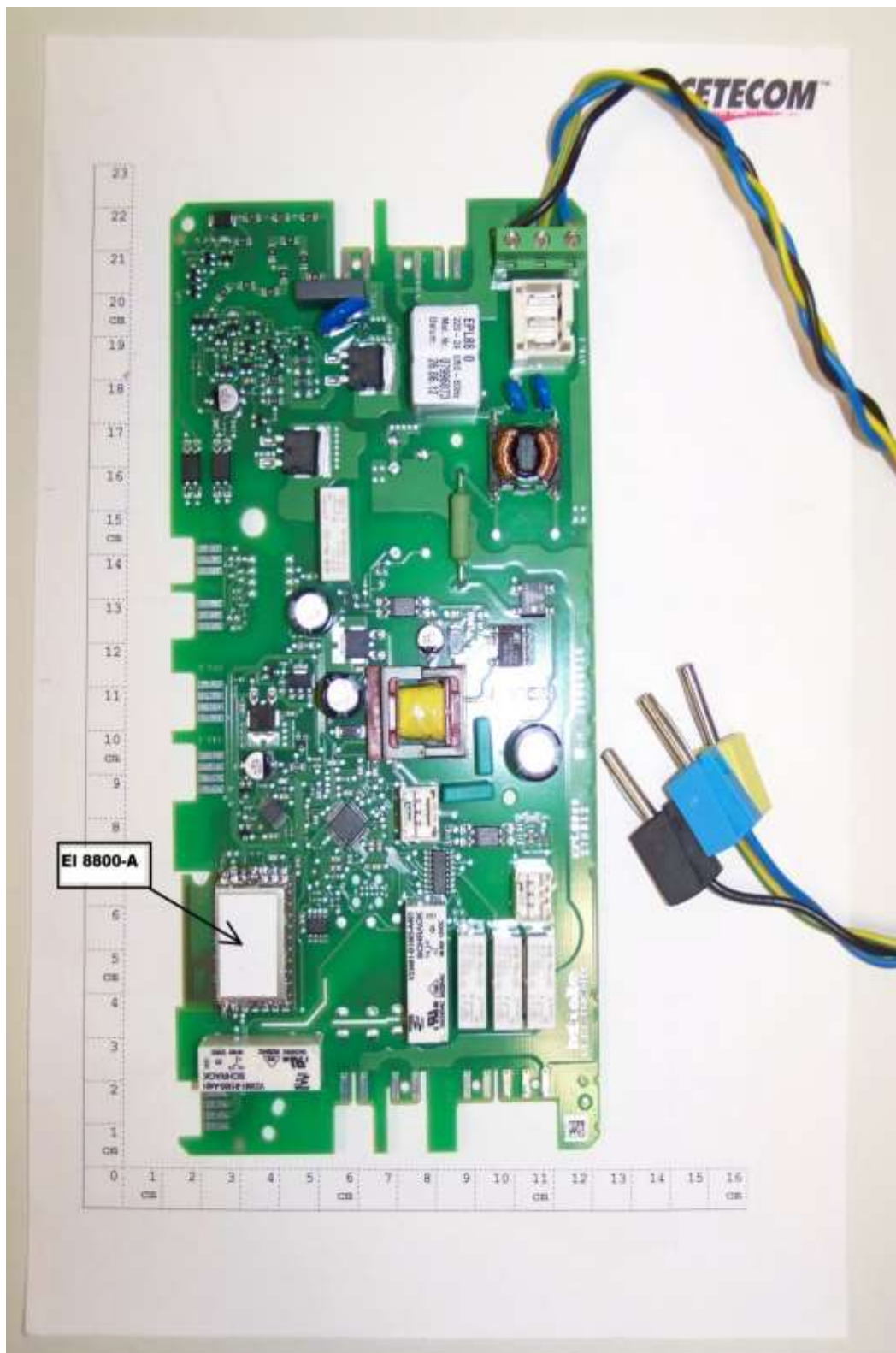
EUT C soldered on AE 1 (PCB), top view. RF module (EUT C) marked at the bottom left.
