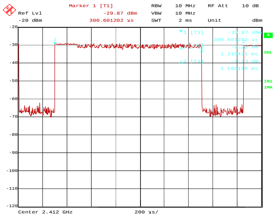
EK037_DutyCycle_ch1_11M_Pos3.wmf: Duty Cycle measurement 802.11b 11 Mbps
