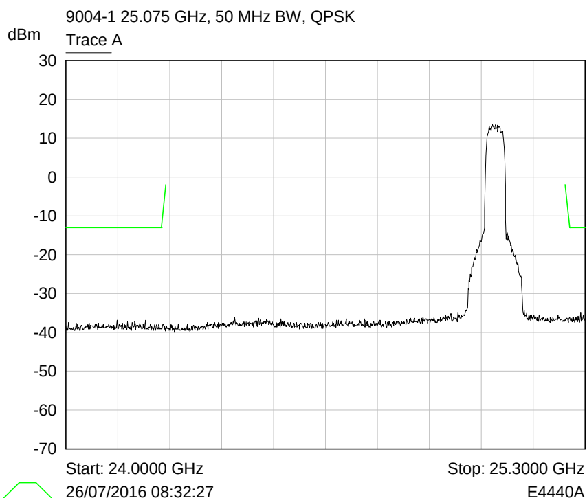
Plot for band edge mask
