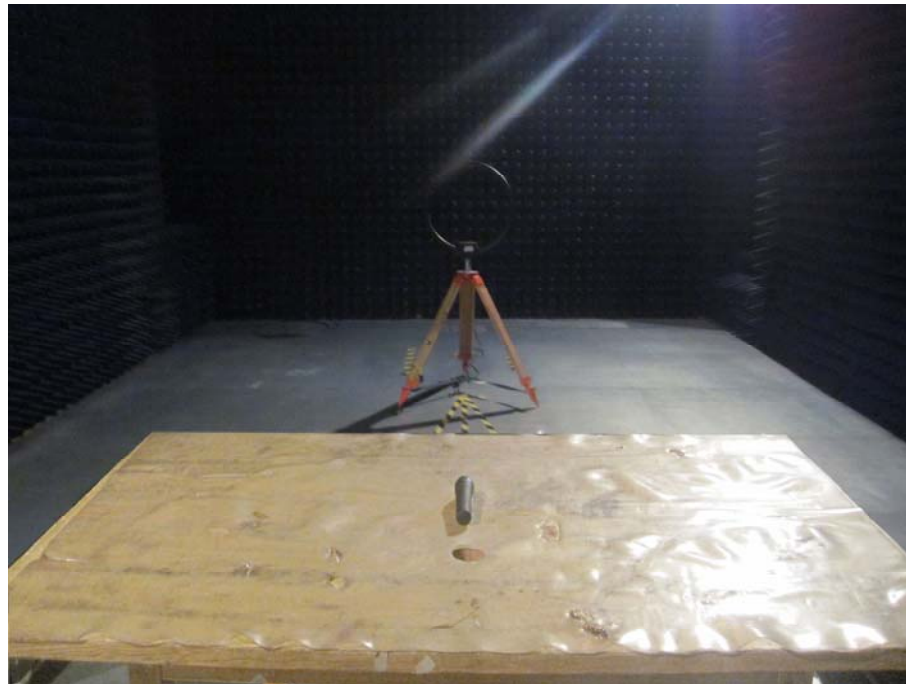
Photograph – Radiation Spurious Emission Test Setup Mode: BT transmitting
