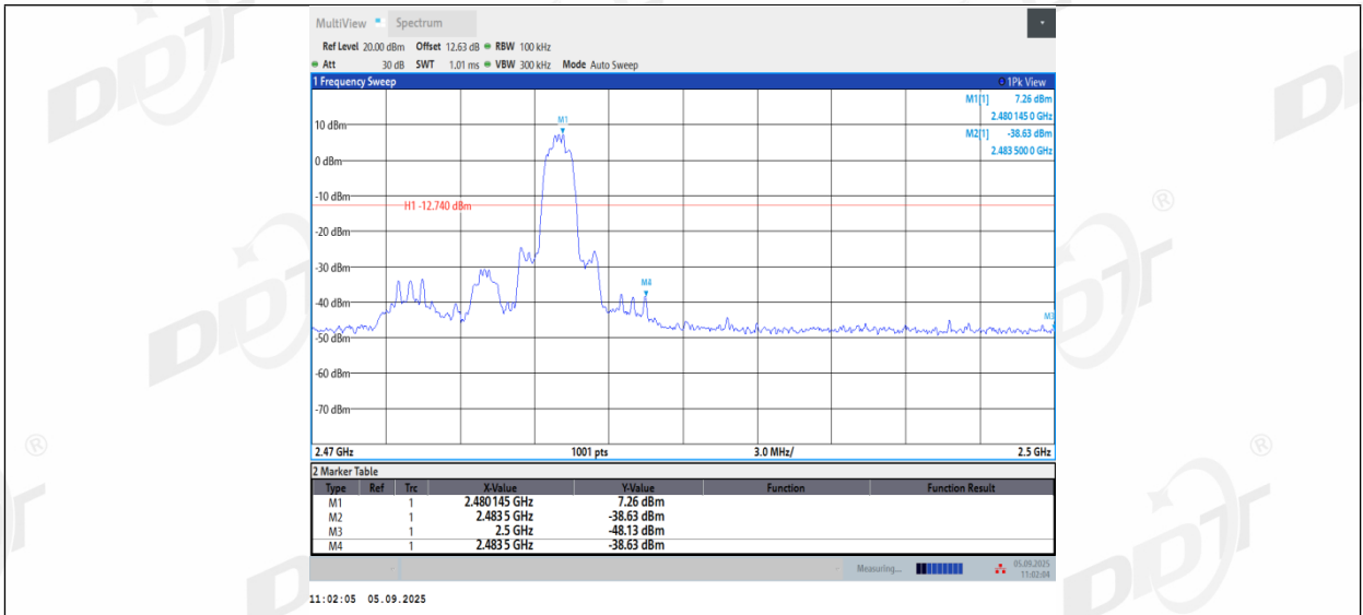
3DH5_Ant2_High_2480
