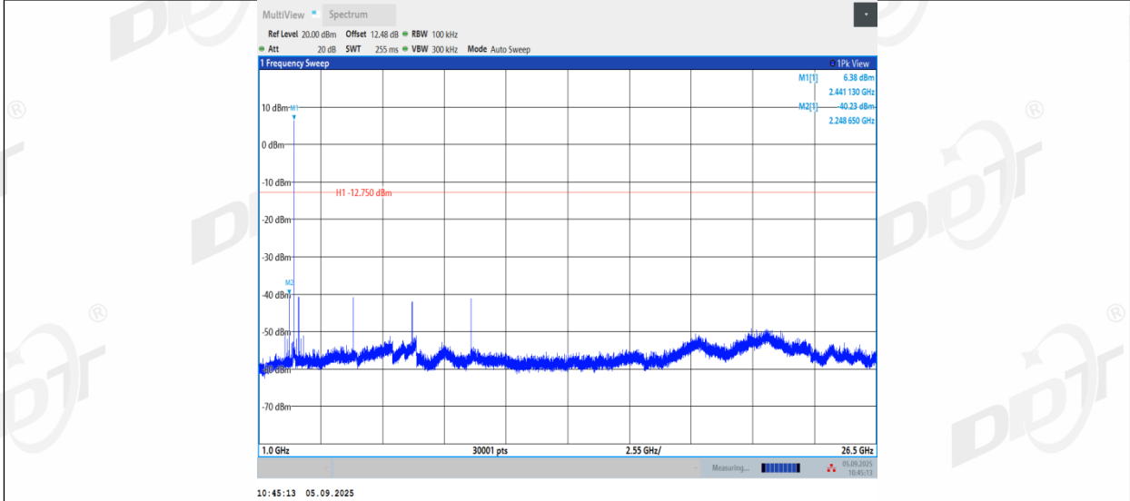
DH5_Ant2_2441_0~Reference
