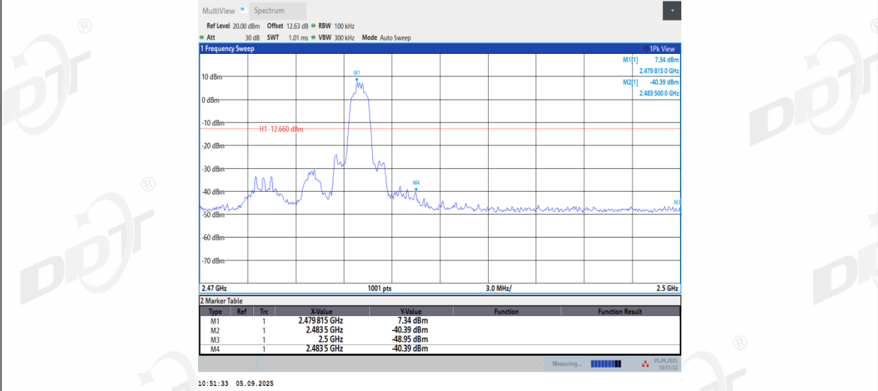
2DH5_Ant2_High_2480
