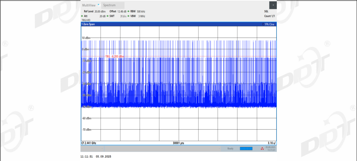
2DH3_Ant2_Hop
