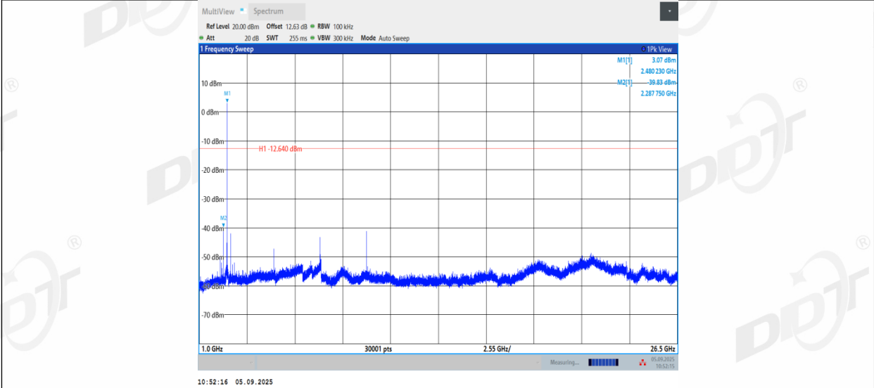
2DH5_Ant2_2480_0~Reference
