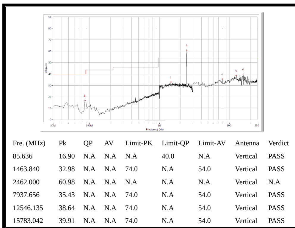
(Plot I.3: Antenna Vertical, 30MHz to 25GHz)
