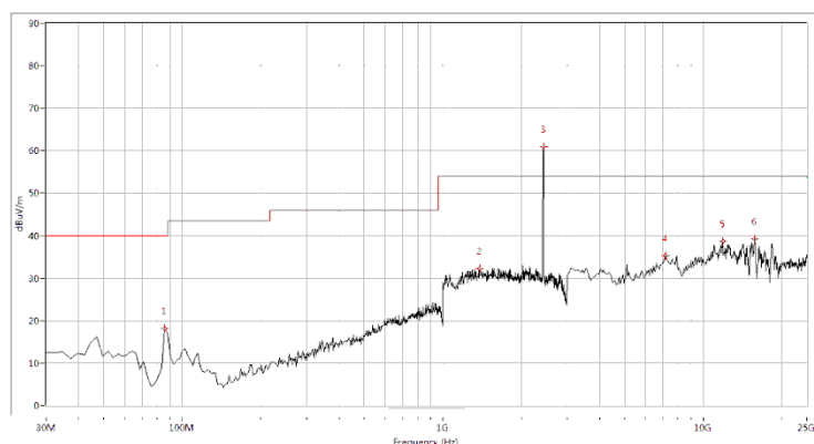
(Plot H.2: Antenna Horizontal, 30MHz to 25GHz)
