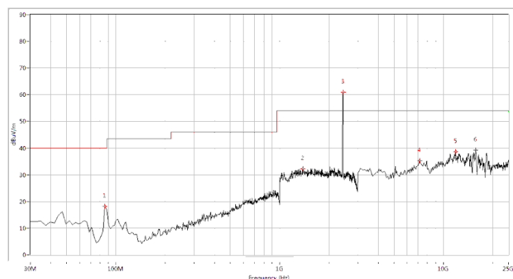
(Plot H.2: Antenna Horizontal, 30MHz to 25GHz)
