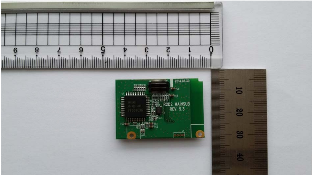
View of Main sub Board (TOP)
