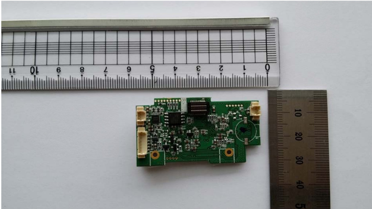
View of Main Board (TOP)
