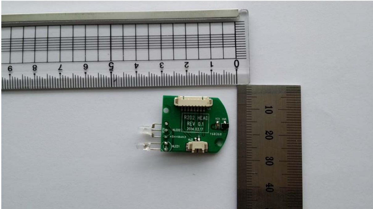
View of Head Board (TOP)
