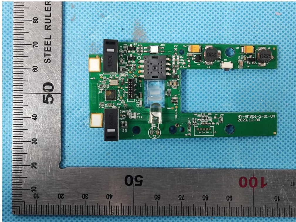
INTERNAL VIEW OF EUT (FIGURE 2 Main PCB Wireless)
