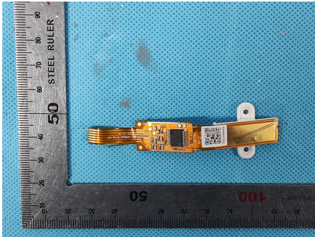
INTERNAL VIEW OF EUT (FIGURE 6 Touch-Scroll)
