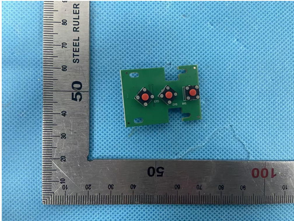
INTERNAL VIEW OF EUT (FIGURE 3 3-Button Scroll)
