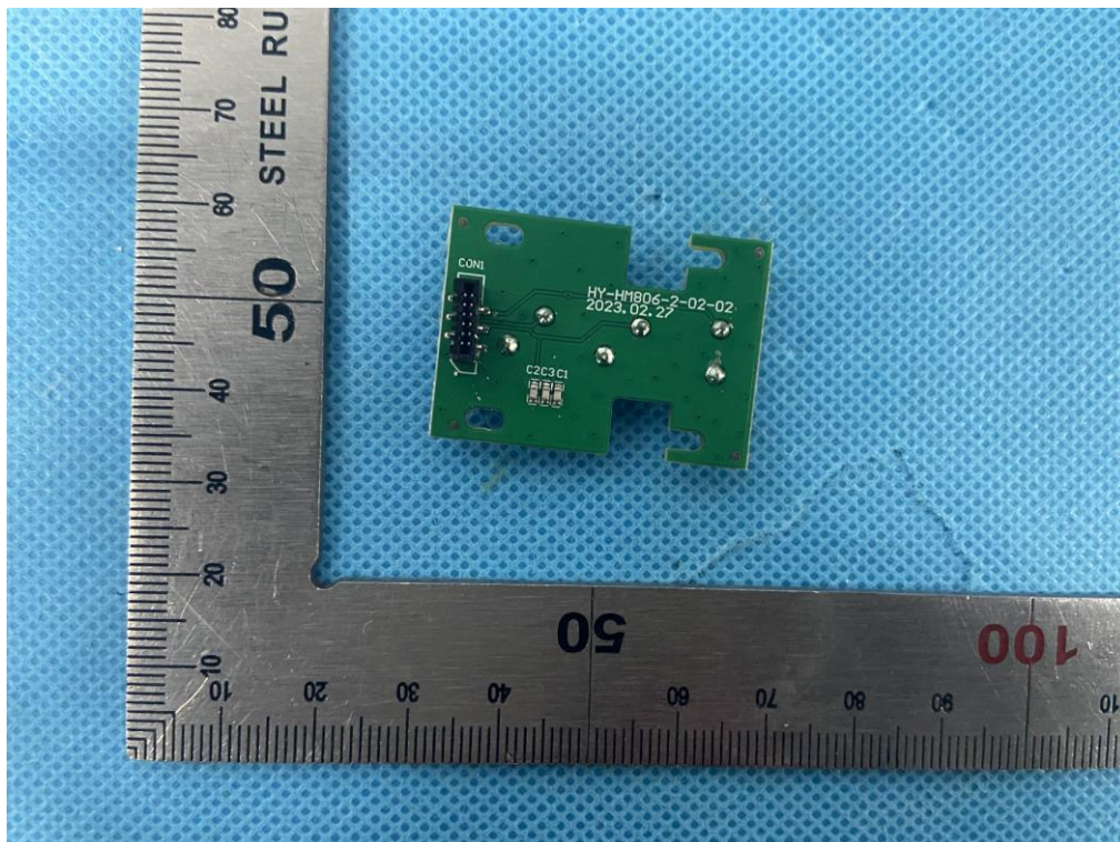
INTERNAL VIEW OF EUT (FIGURE 4 3-Button Scroll)
