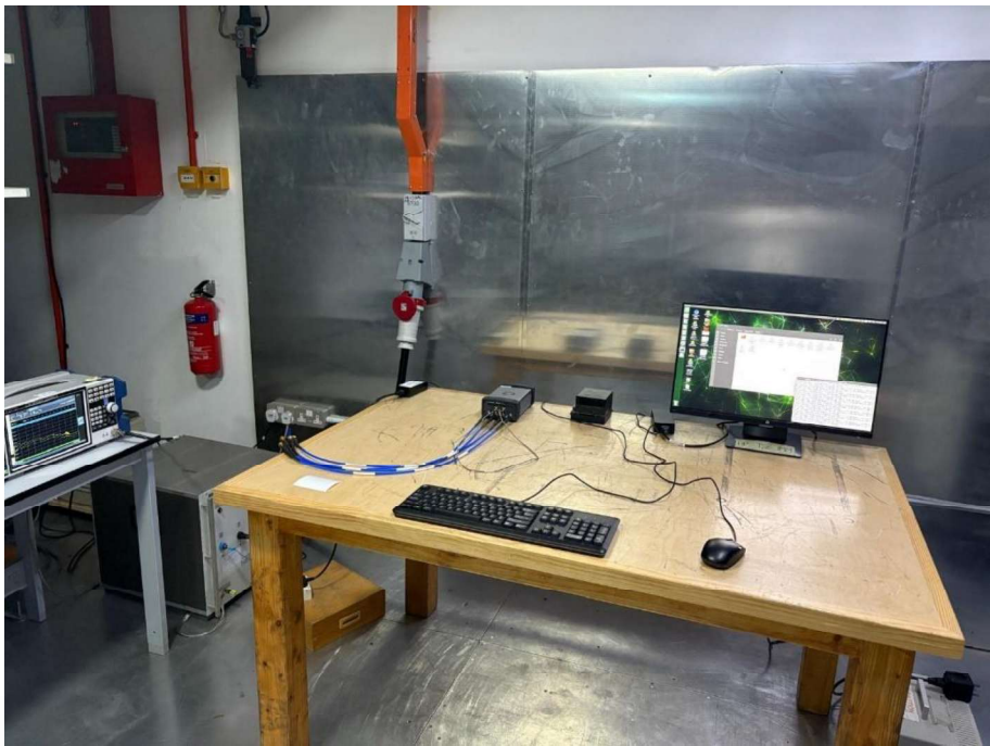
Conducted Emissions at Mains Test Setup (Front View)
