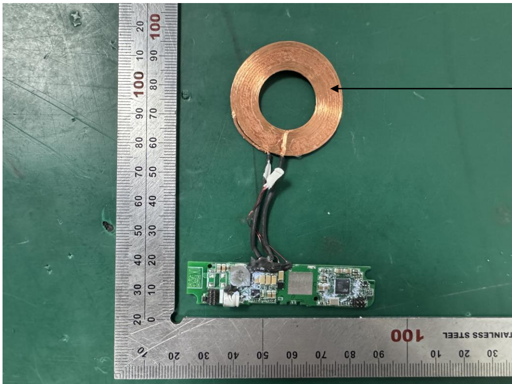
Coil Antenna
