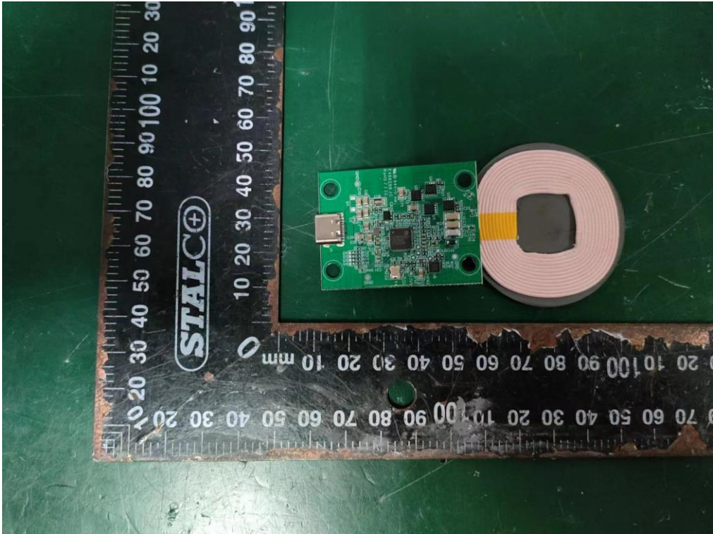
Internal Photos M/N: WRLS-PAD-15W
