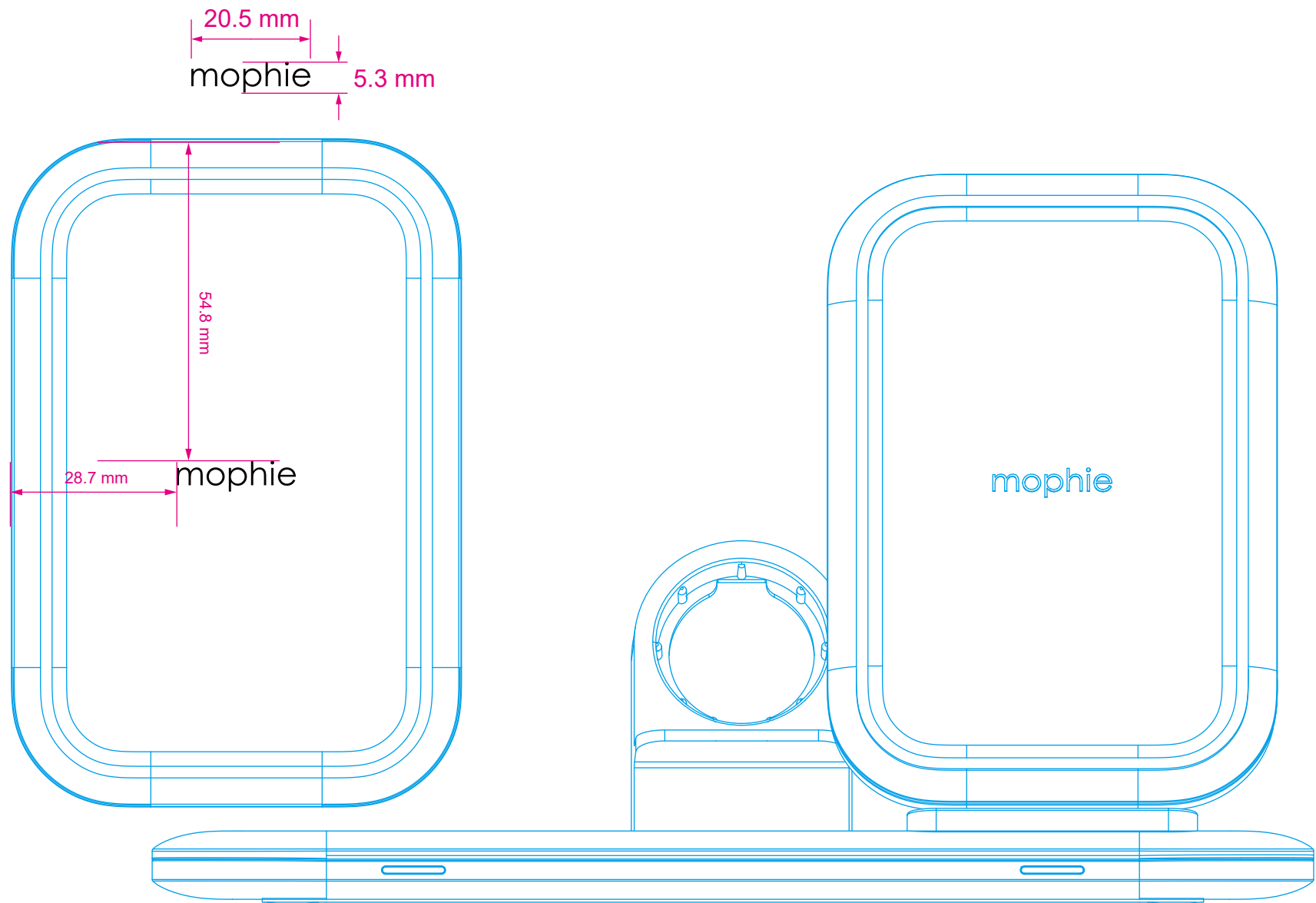
front view
