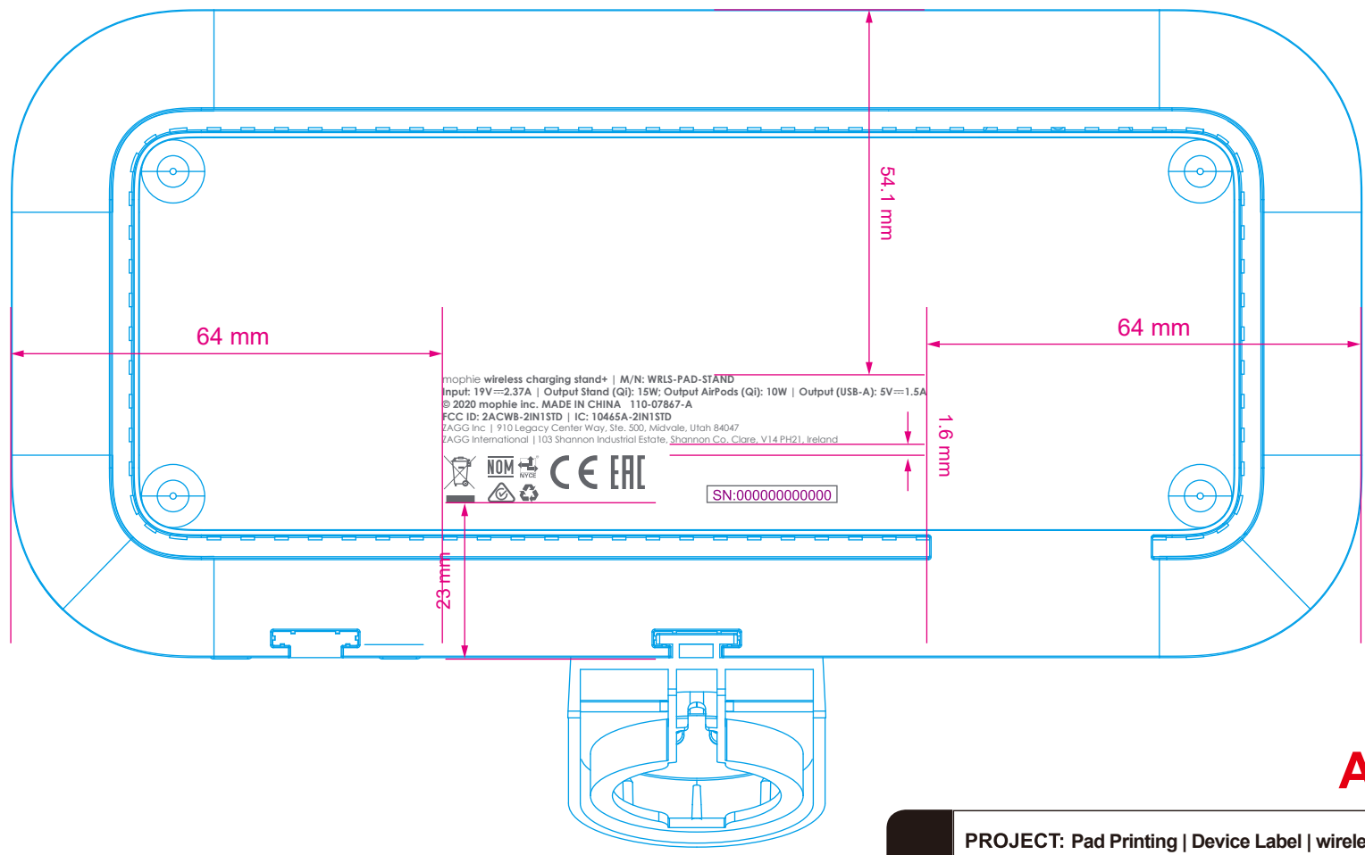
bottom view
