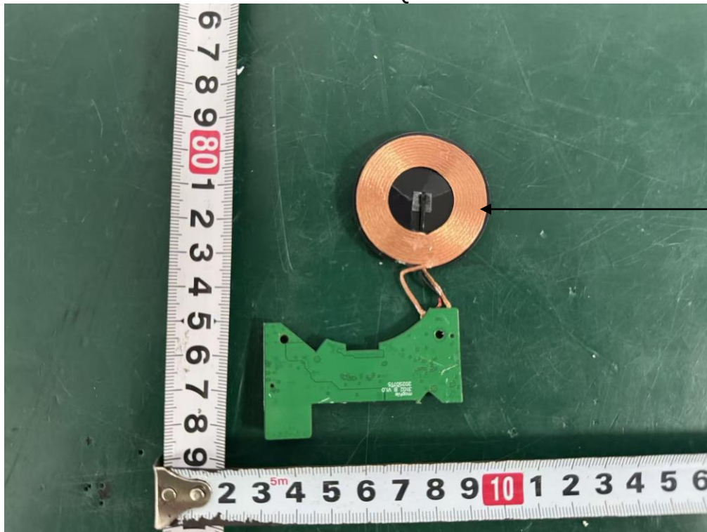
AirPods Coil Antenna
