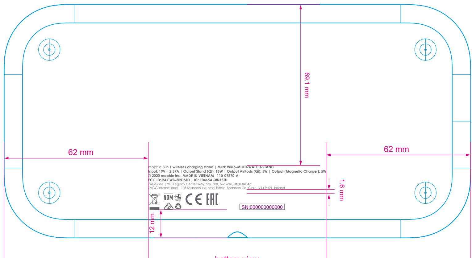
bottom view
