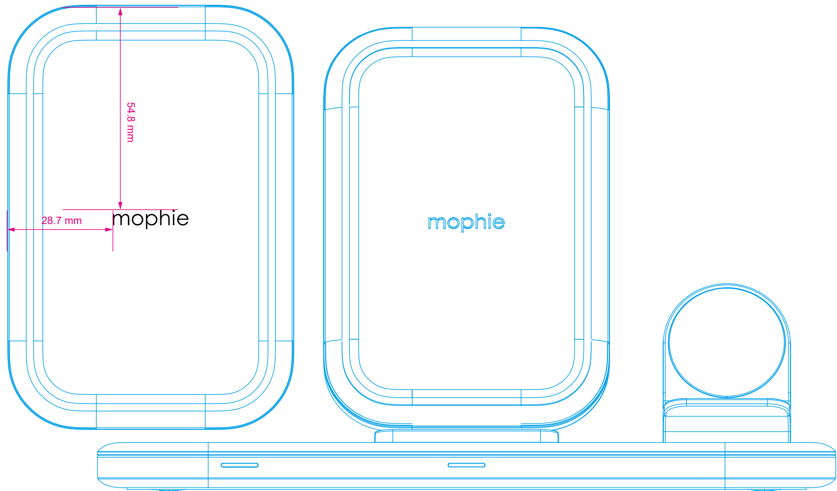
front view
