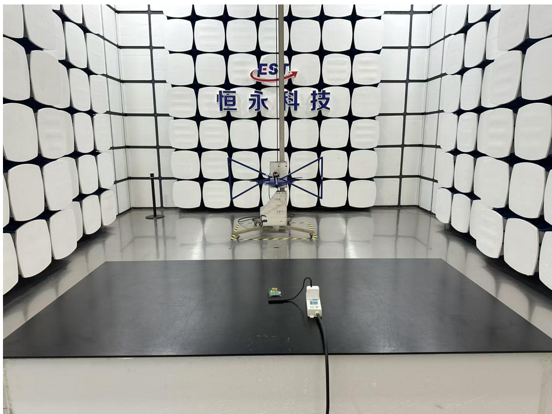
Radiated Test (Above 30MHz)
