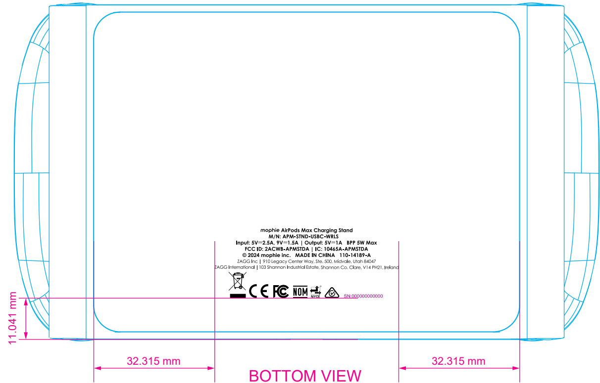
BOTTOM VIEW
