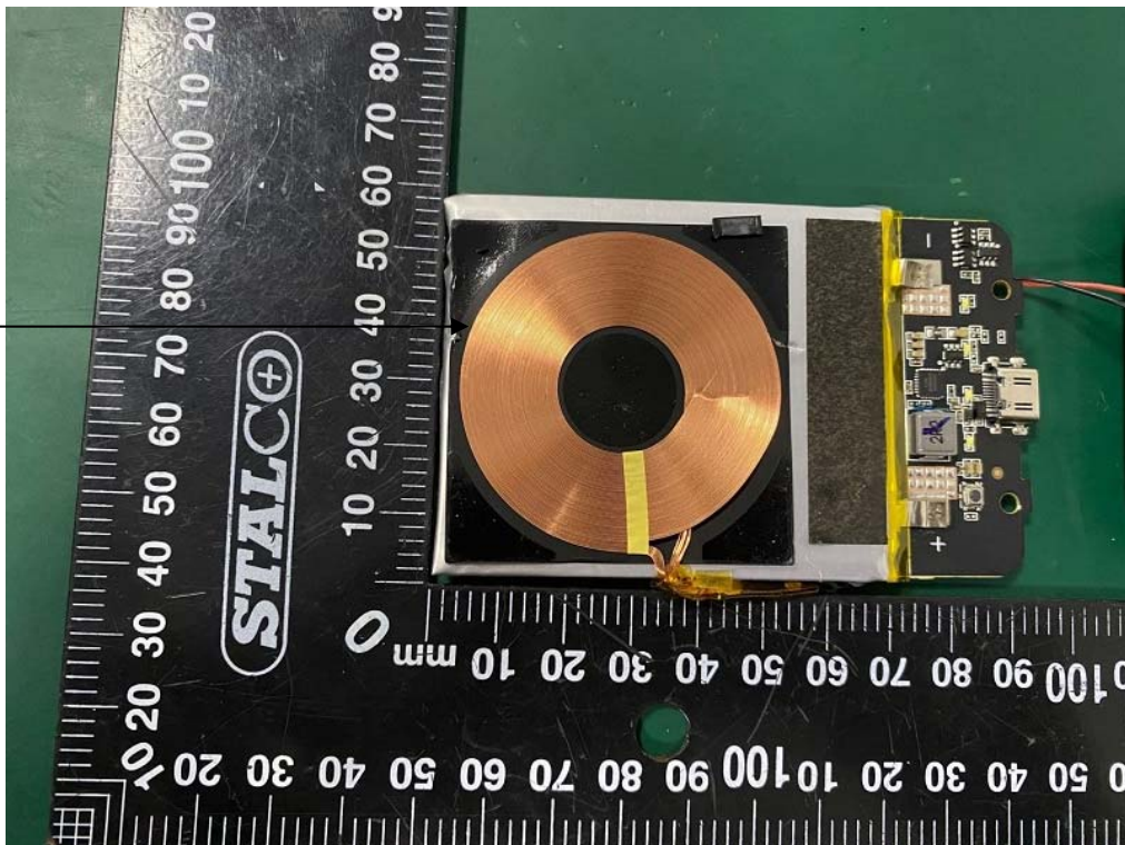
RX Coil Antenna
