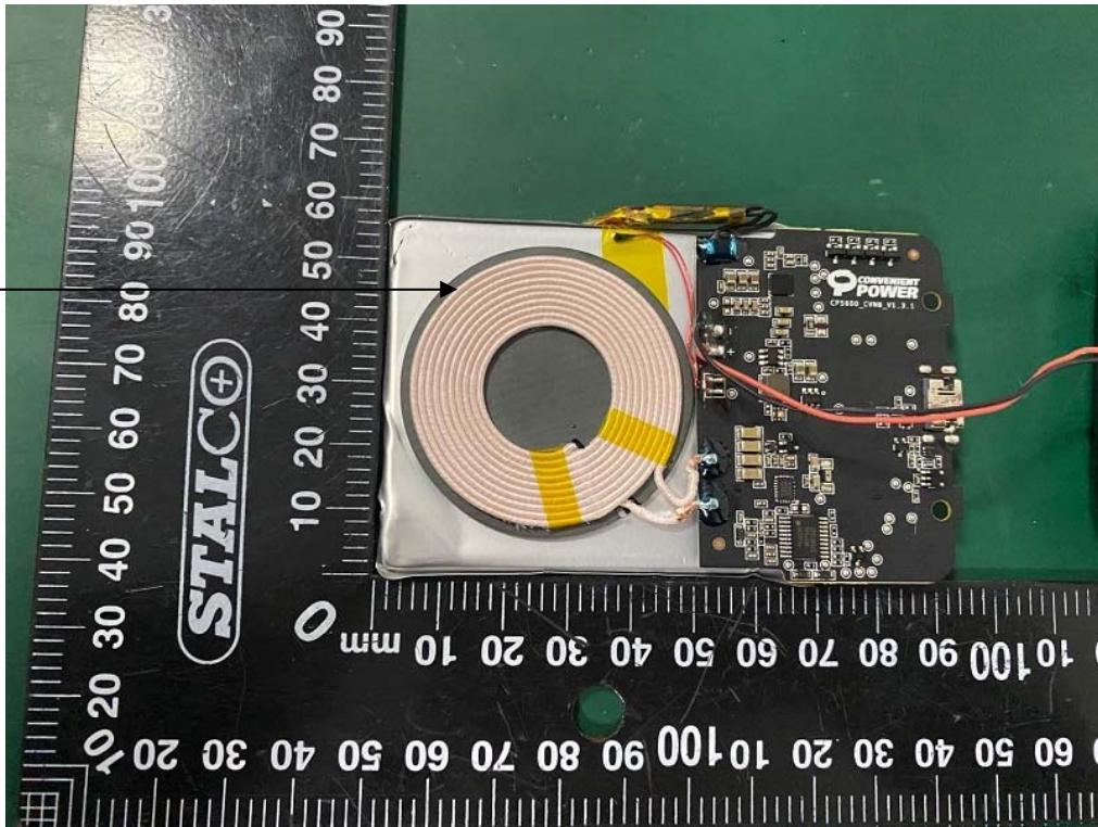
TX Coil Antenna
