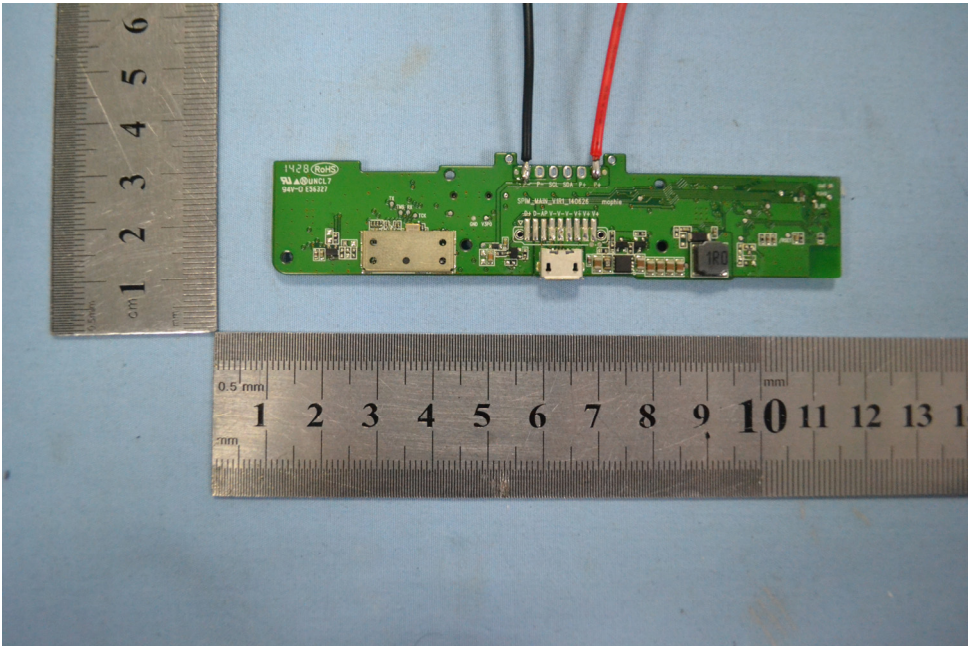
Solder Board-Component View 1
