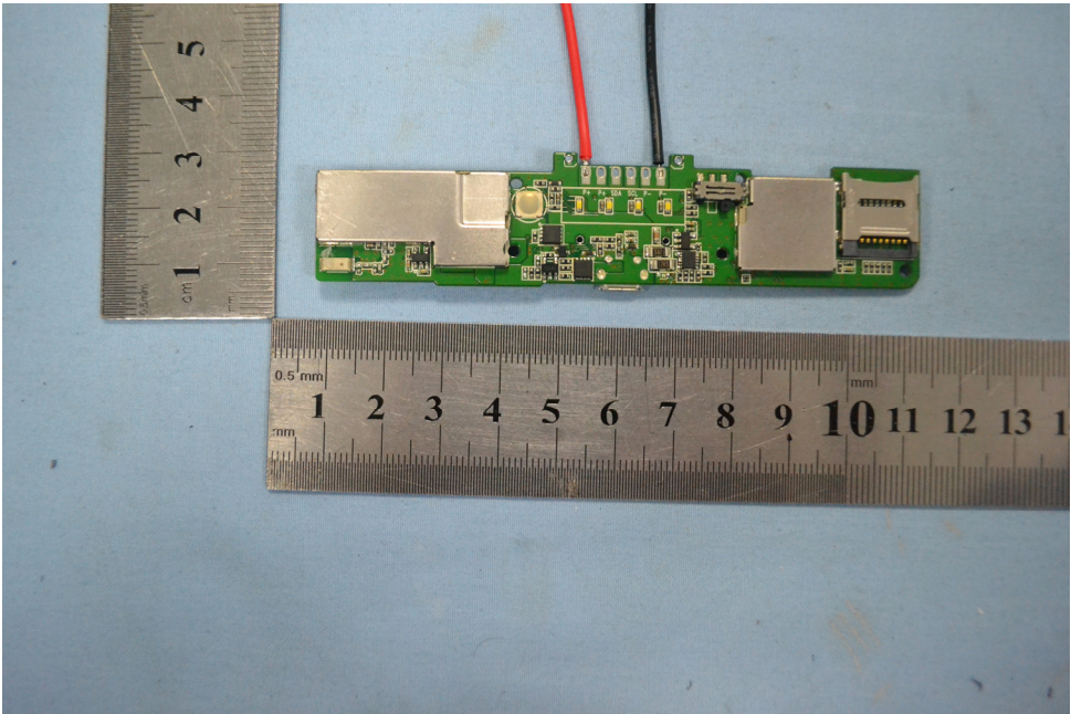
Solder Board-Component View 3
