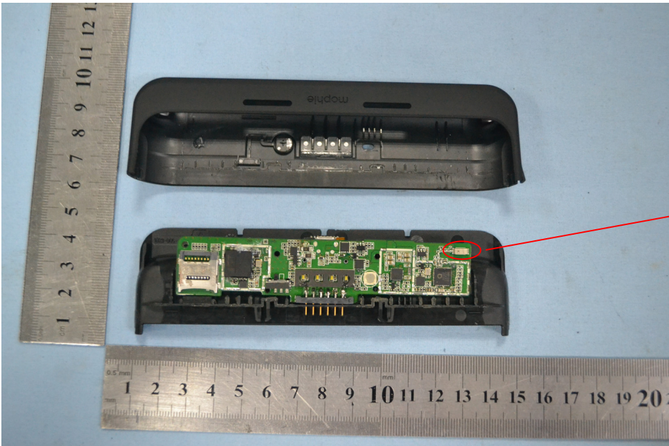
EUT Housing and Board View 2
