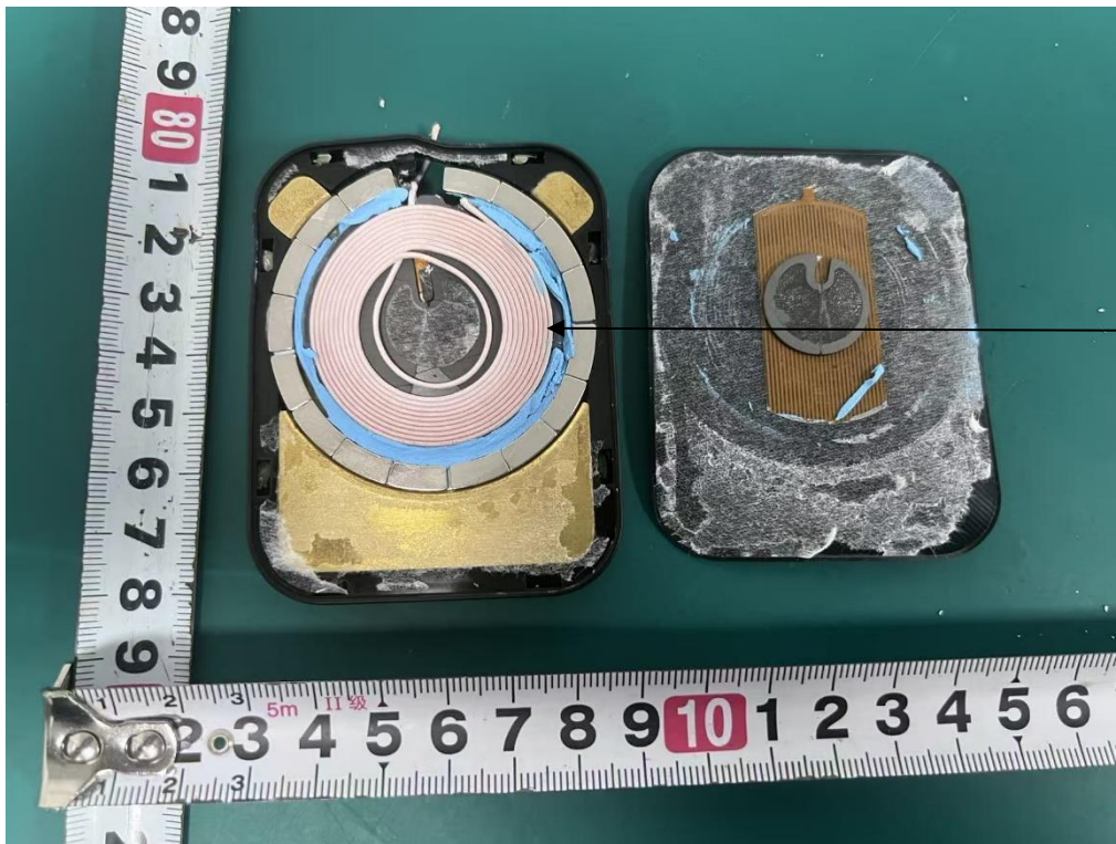
Coil Antenna
