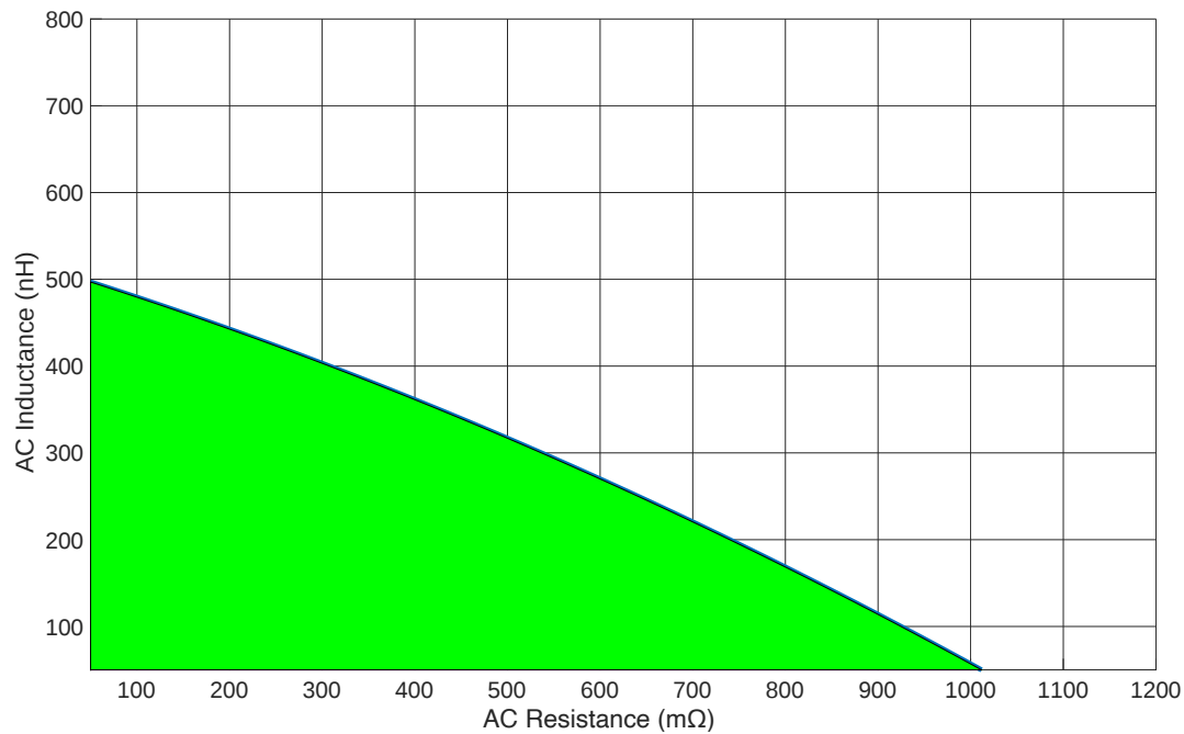
Figure 72-3 Watch Fast Charger Module cable requirements at 326.5 kHz
