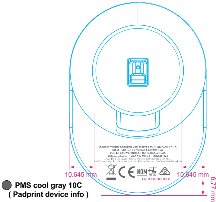
back view
