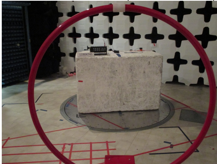
RADIATED EMISSIONS BELOW 30MHz (FRONT – WITH 15W LOAD)
