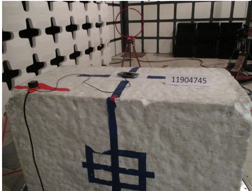
RADIATED EMISSIONS BELOW 30MHz (BACK - WITH REAL PHONE)
