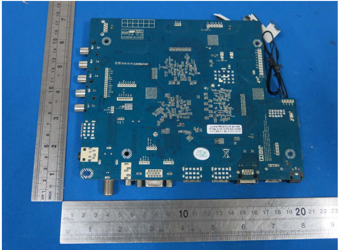
Mainboard with USB 3.0 Port
