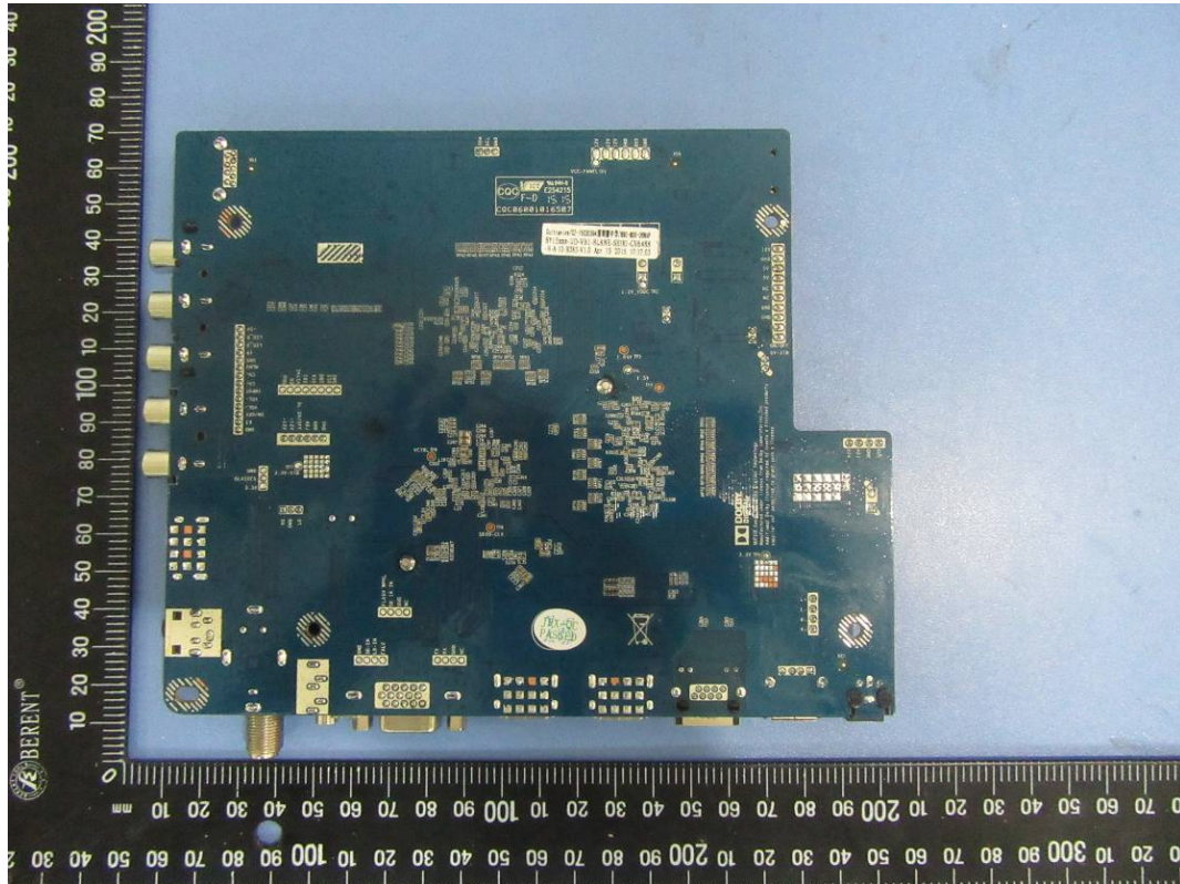
Mainboard without USB 3.0 Port
