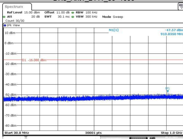
DH5_Ant1_2441_30~1000
