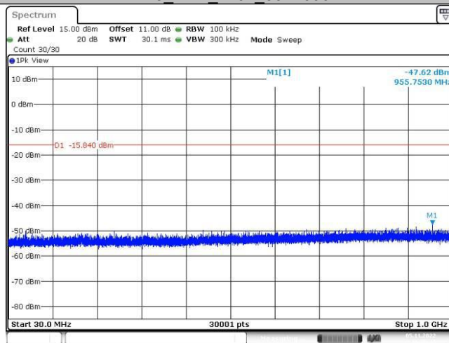
DH5_Ant1_2402_30~1000
